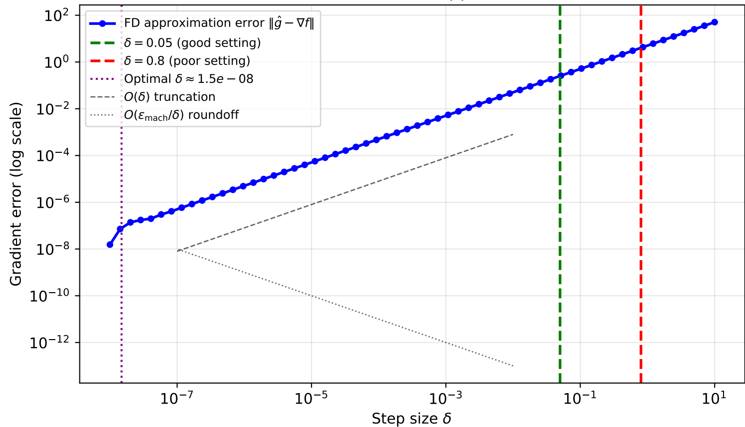
Q4: Finite Difference Gradient Approximation Error vs \delta
