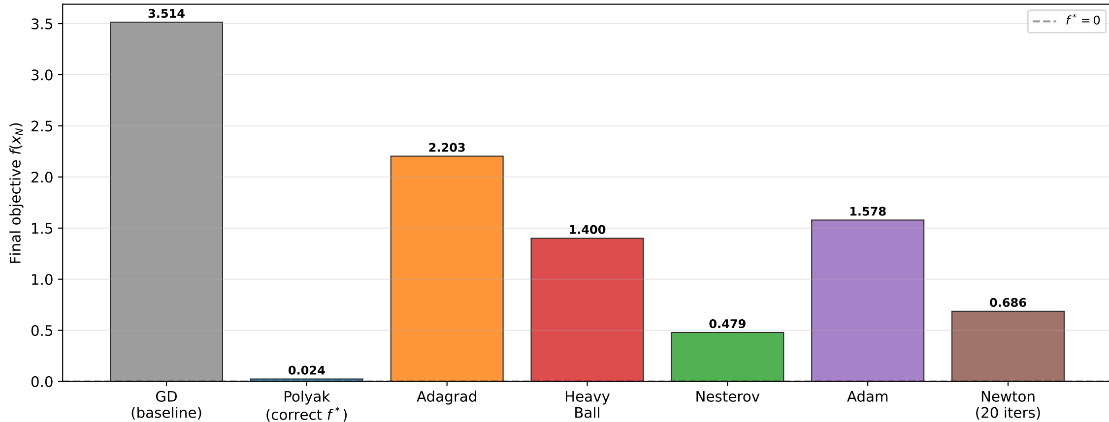
Benchmark C (Rosenbrock): Final Objective — Q1/Q2/Q3 Methods Comparison
