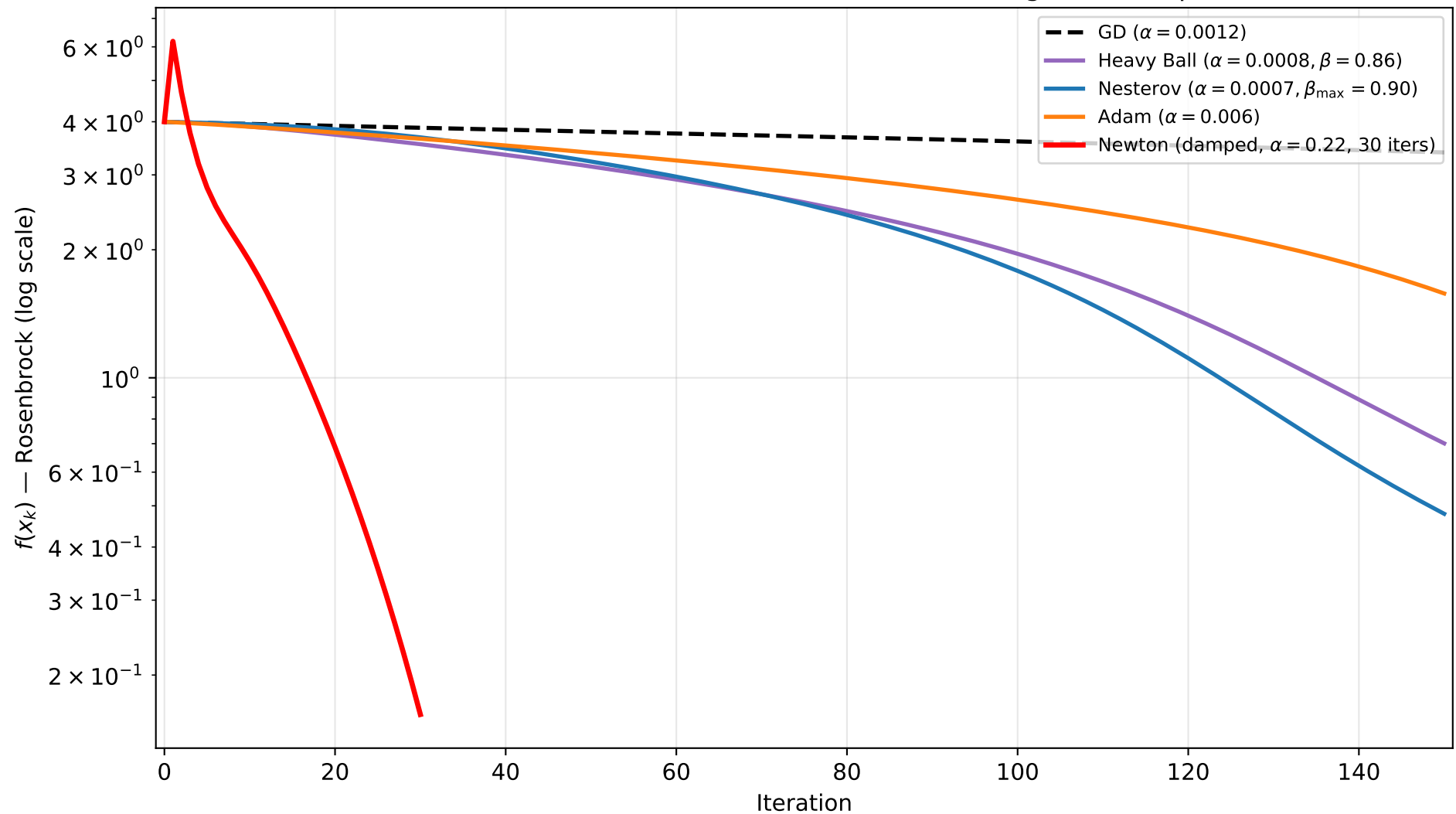
All Methods on Rosenbrock (Benchmark C): Convergence Comparison
