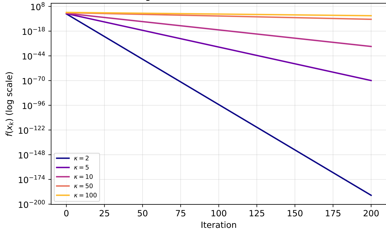
GD Convergence vs Condition Number (Quadratic)
