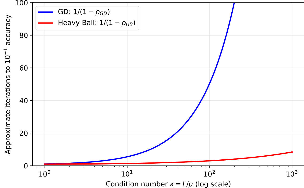
Effective Iterations vs Condition Number
