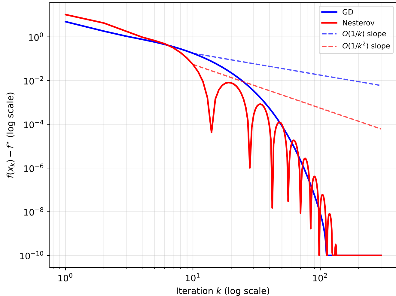
Benchmark B: Convergence Rate (log-log)
