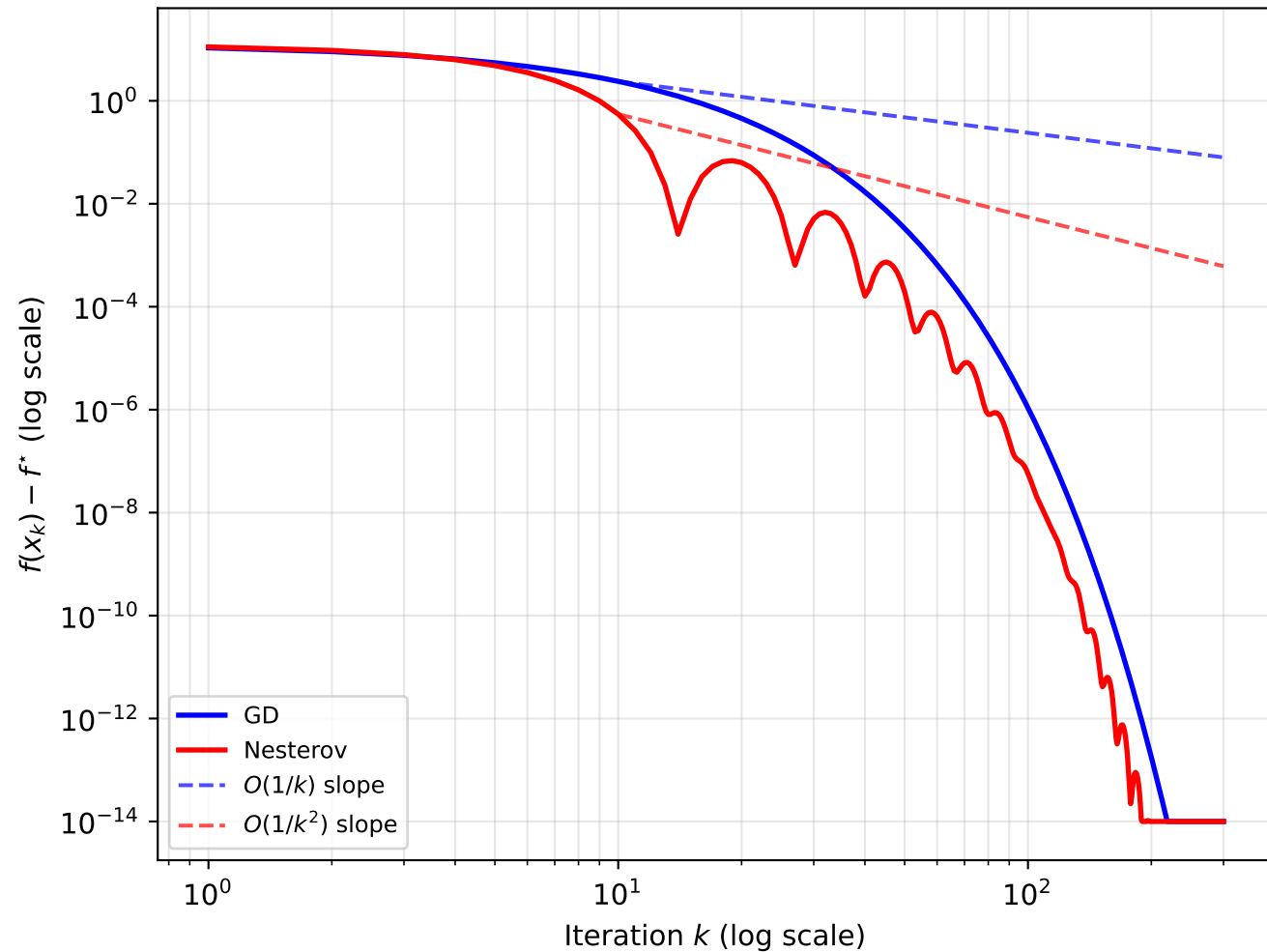
Benchmark A: Convergence Rate (log-log)
