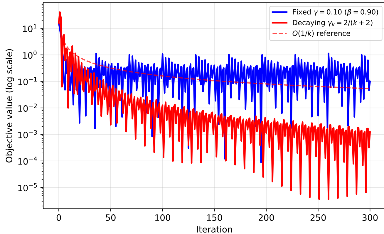
FW: Fixed vs Decaying Step Size
