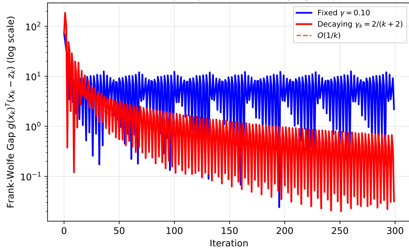
FW Duality Gap: Fixed vs Decaying Step
