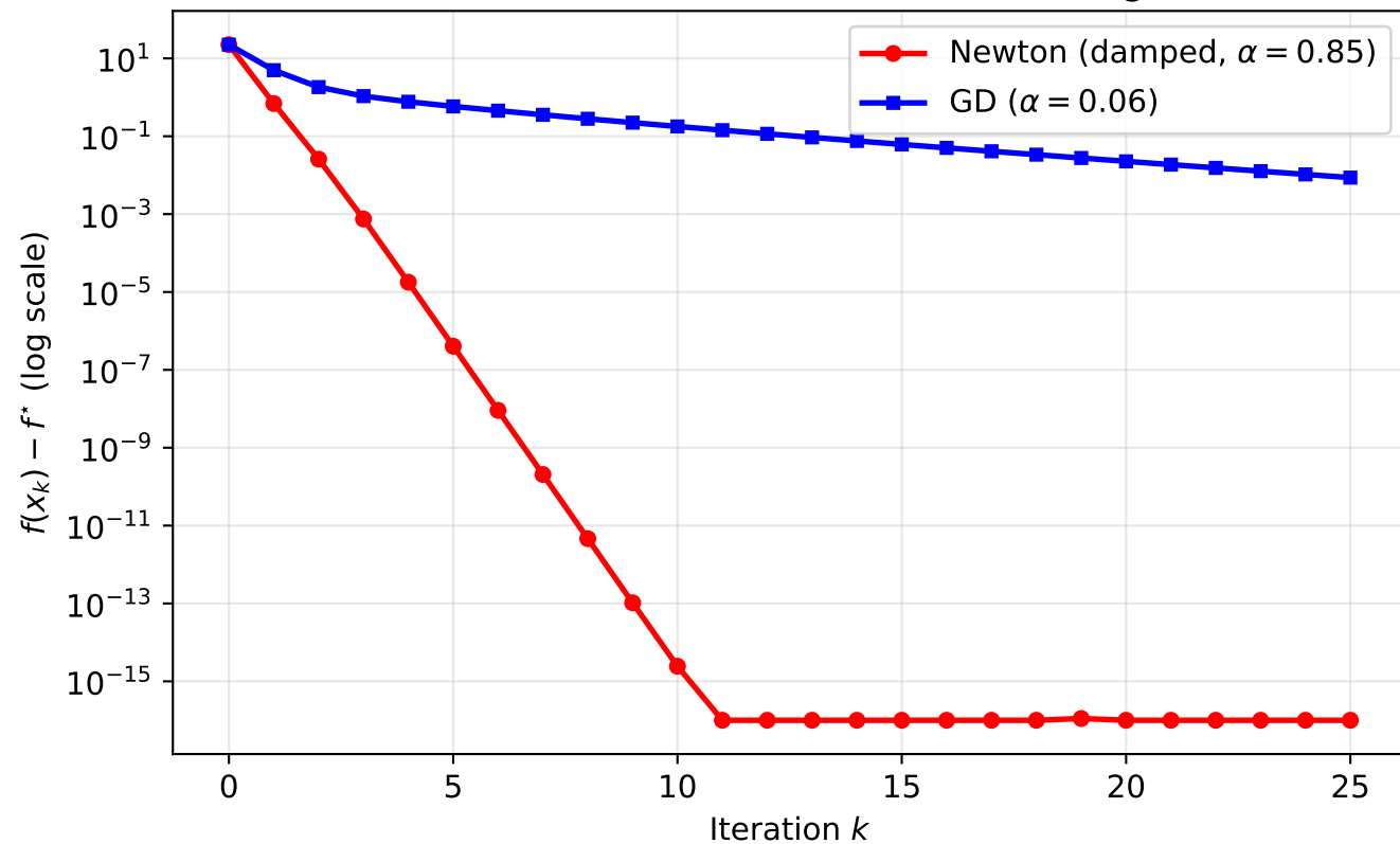
Newton vs GD: Benchmark B (semi-log)
