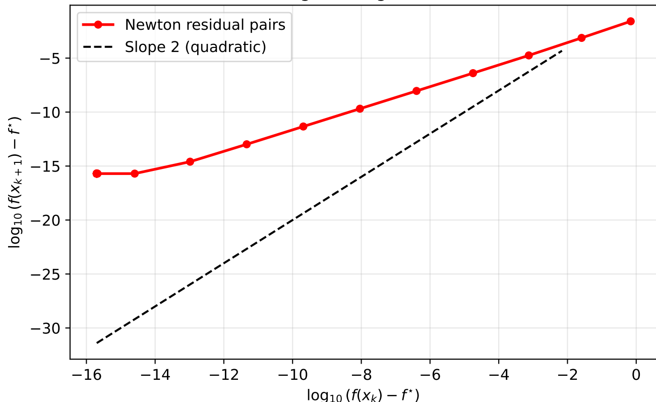
Quadratic Convergence Signature (Benchmark B)
