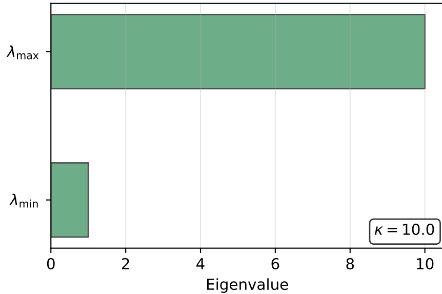
Bench. B: H = \text{diag}(2 - \sin x_1, 10) (moderate anisotropy)
