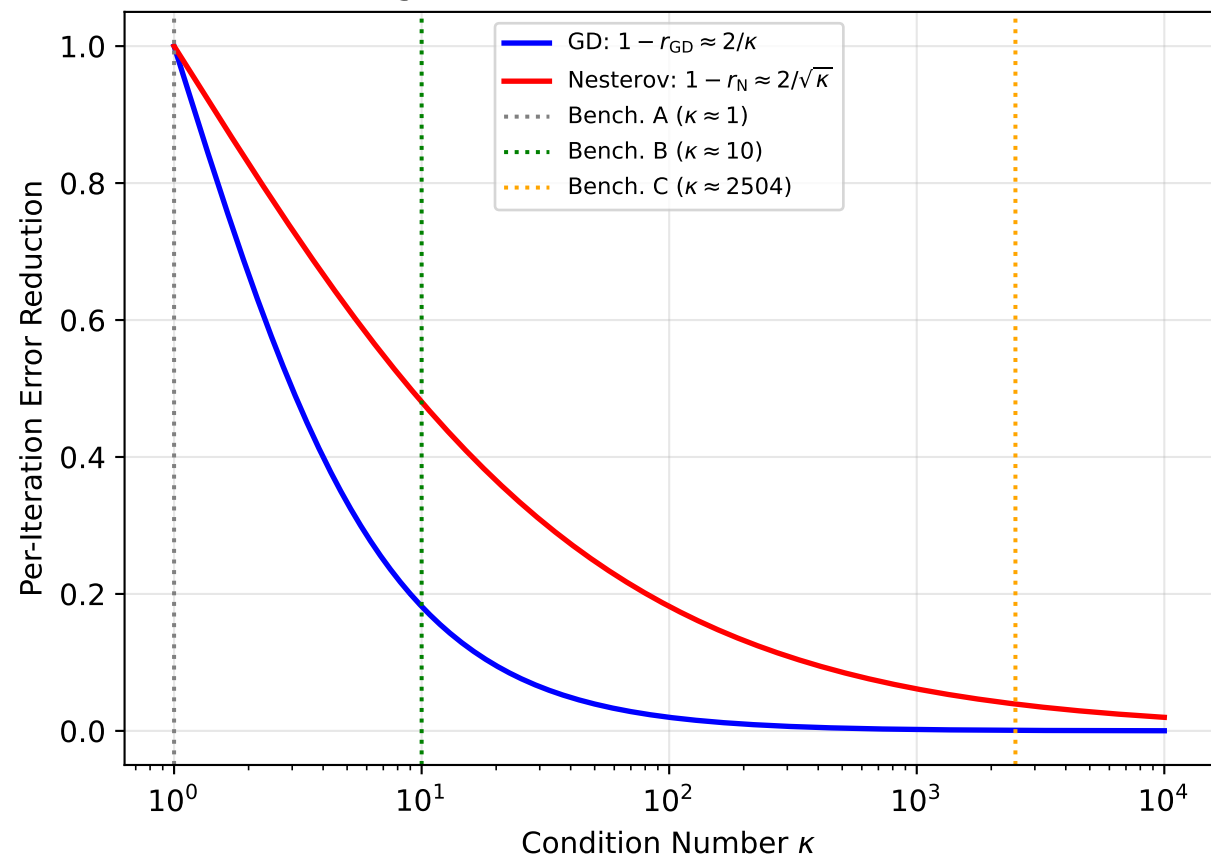
Convergence Rate 1 - r vs Condition Number
