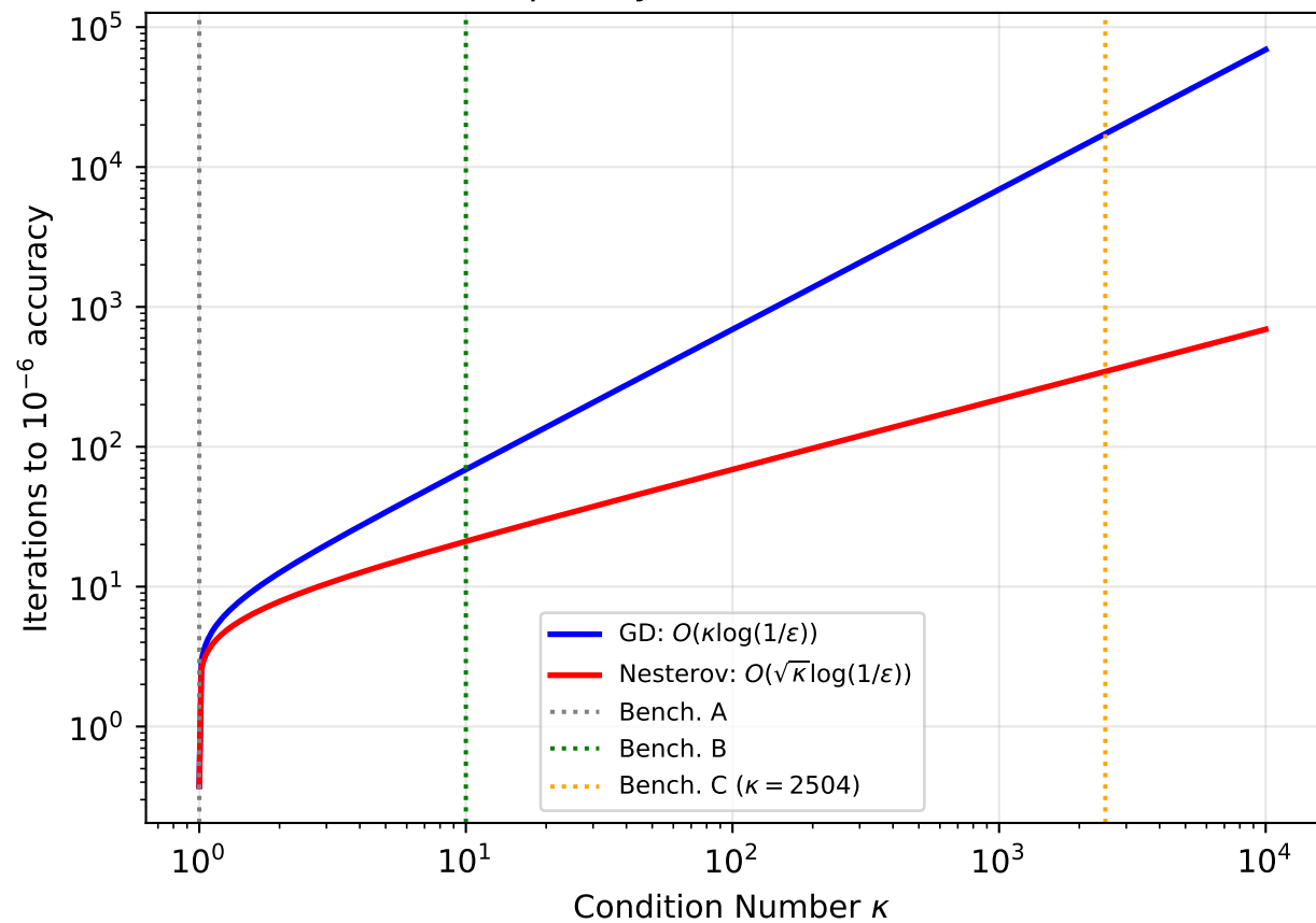
Iteration Complexity vs \kappa (to reach f - f^* < 10^{-6} )
