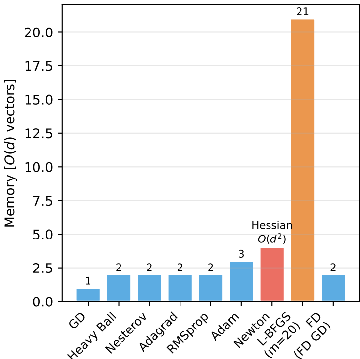
Memory Footprint Comparison
