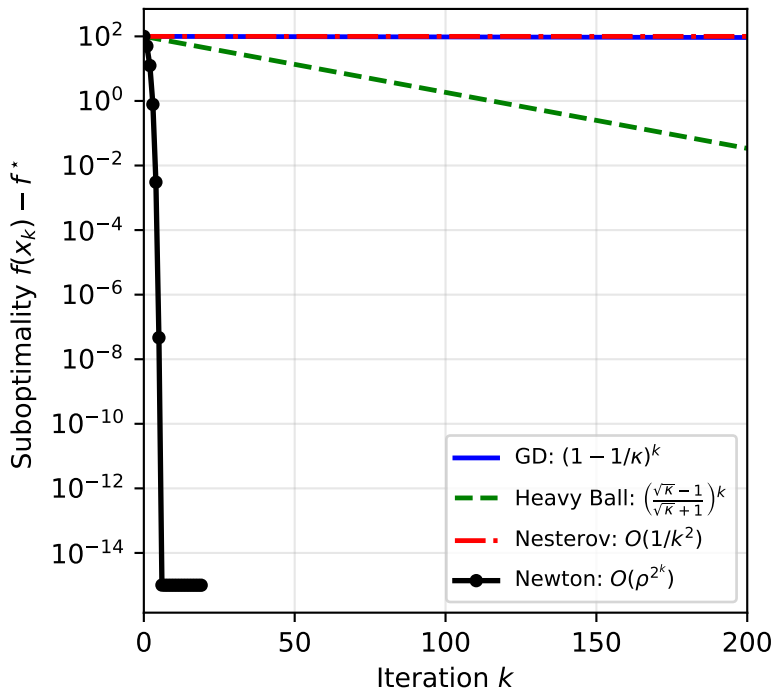
Theoretical Convergence Rates ( \kappa = 2508 )
