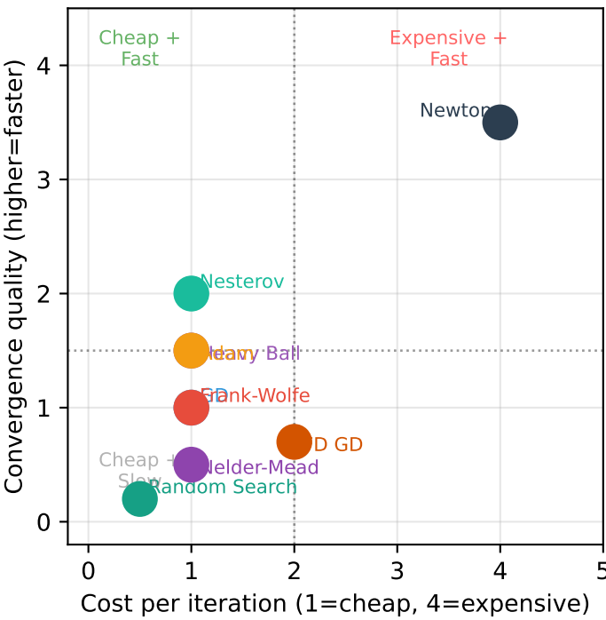
Algorithm Trade-off: Cost vs Convergence
