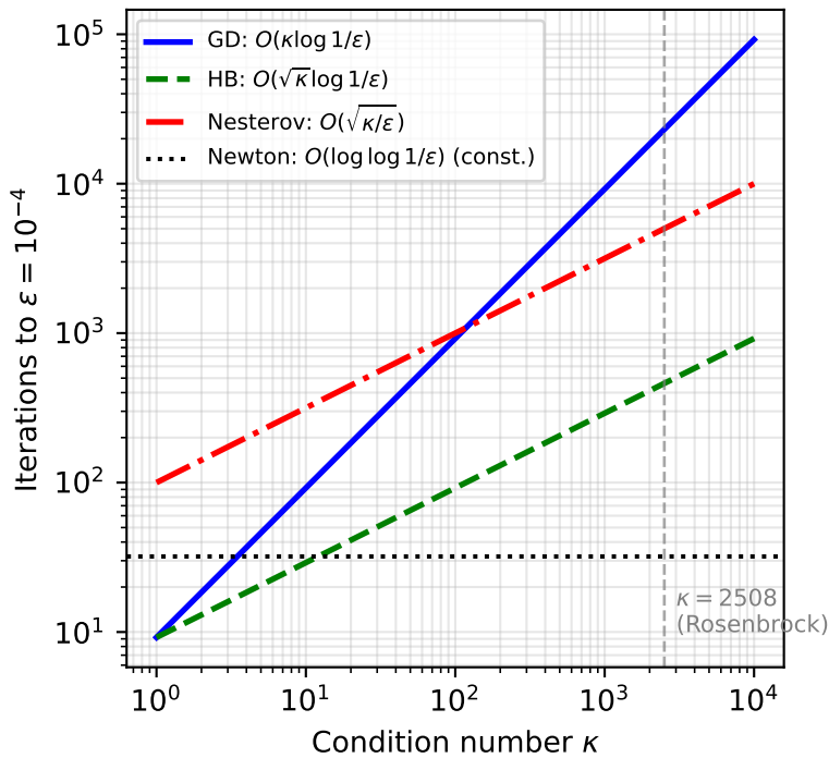
Iteration Count vs Condition Number
