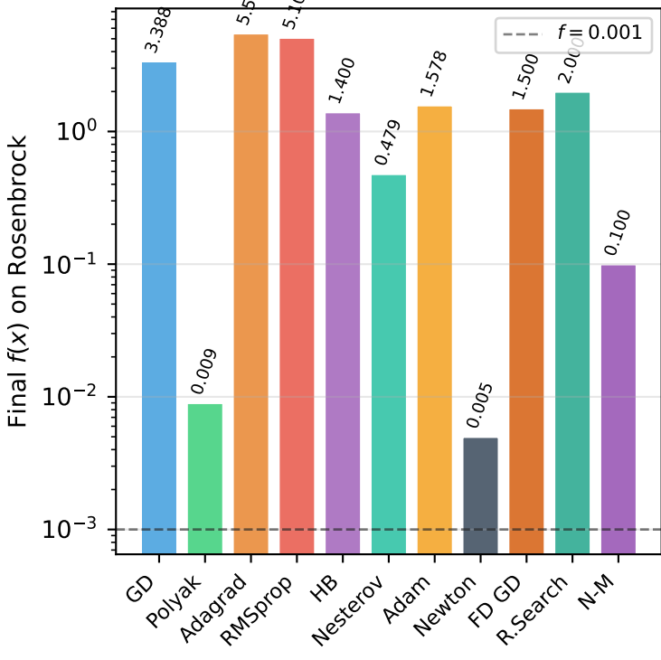
Final Objective: Benchmark C
