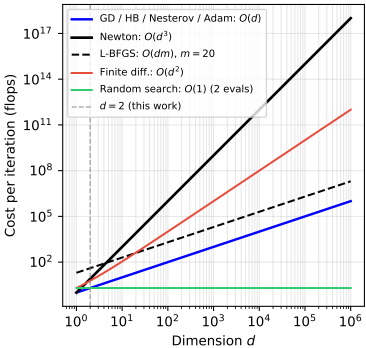
Per-Iteration Cost vs Dimension
