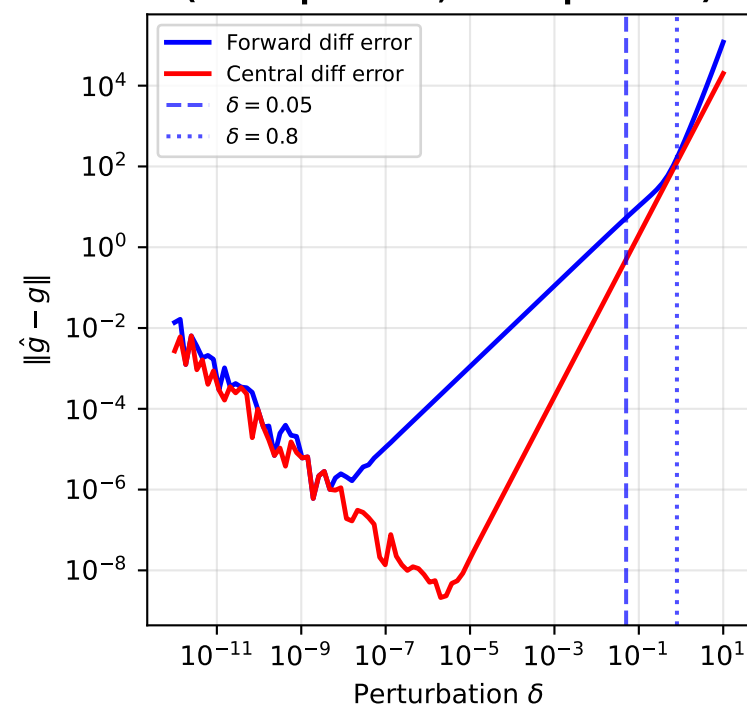
FD vs CD: Gradient Error (FD slope=1.00, CD slope=2.00)
