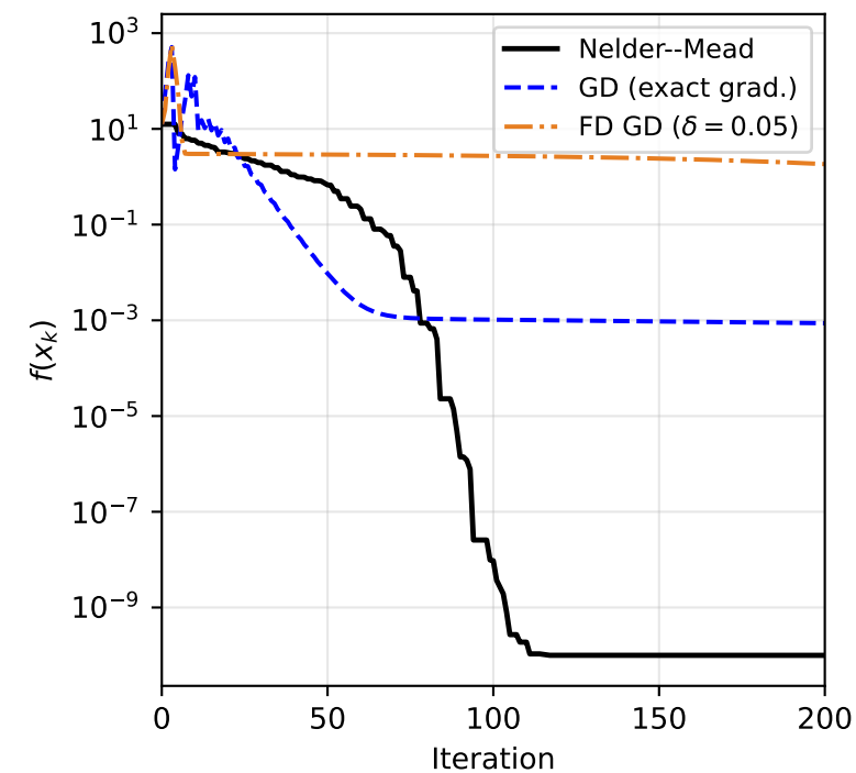
Nelder-Mead vs GD on Rosenbrock
