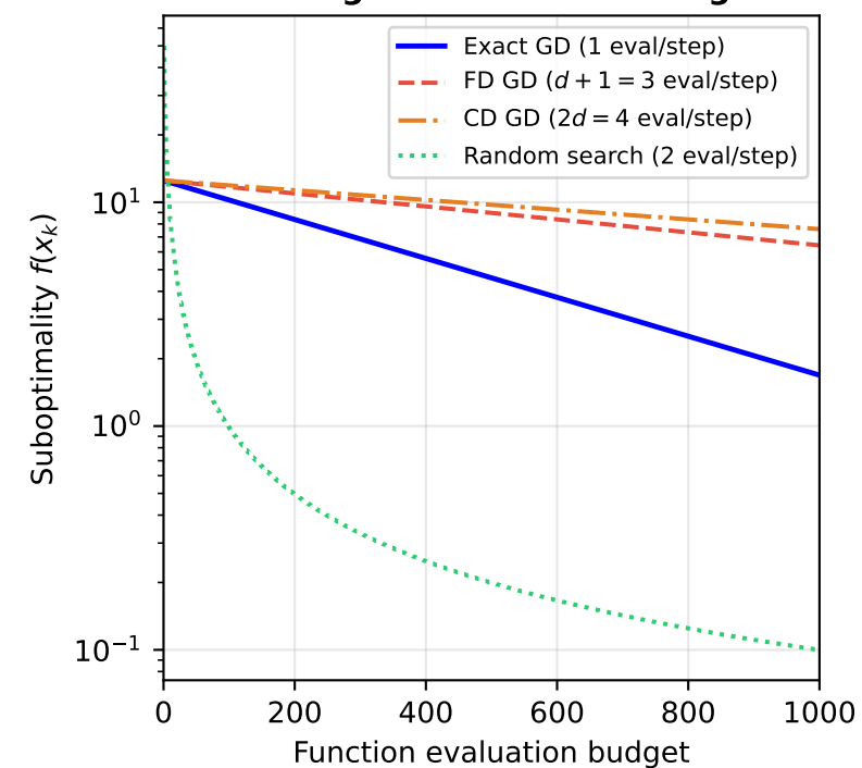
Convergence vs Oracle Budget
