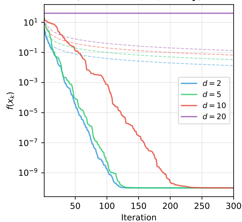
Random Search: O(d/k) Rate vs Dimension (dashed = O(d/k) theory)
