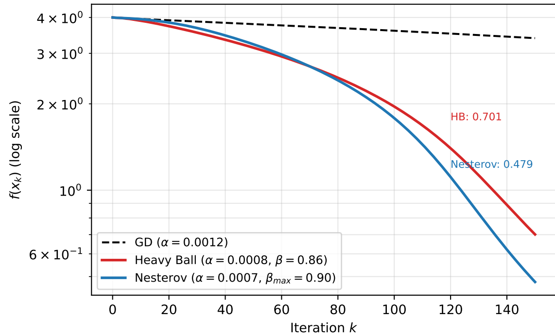
GD vs Heavy Ball vs Nesterov on Rosenbrock ( \kappa \approx 2000 )
