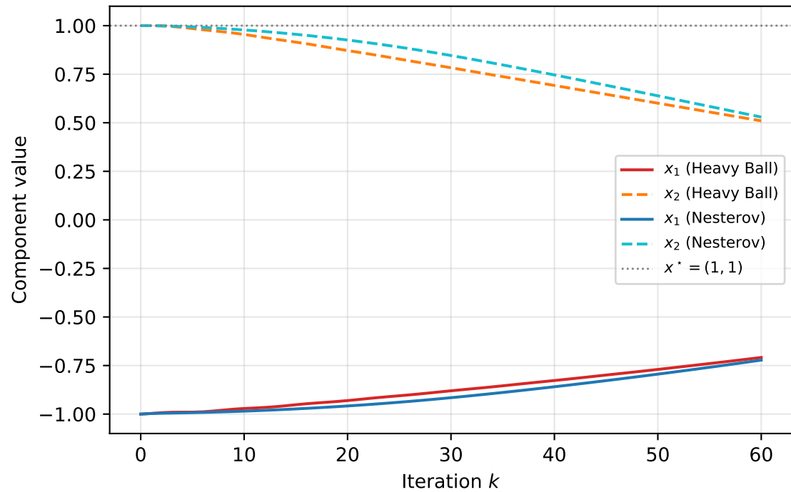
Component Trajectories: Heavy Ball vs Nesterov
