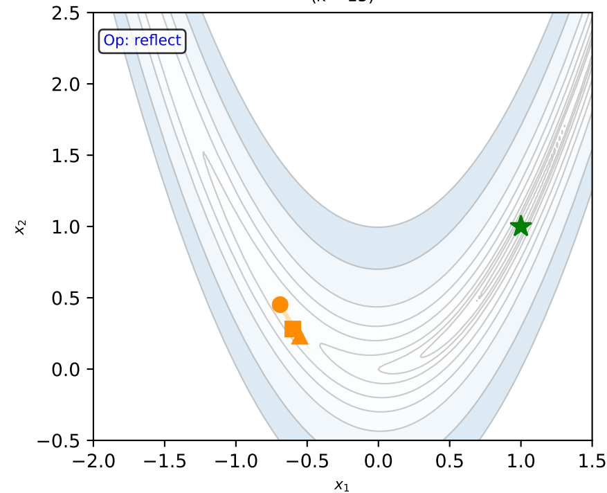
Valley entry ( k = 15 )
