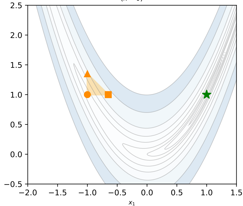
Initial simplex ( k = 0 )
