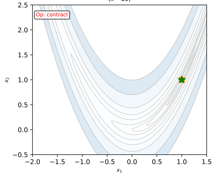
Near optimum ( k = 80 )
