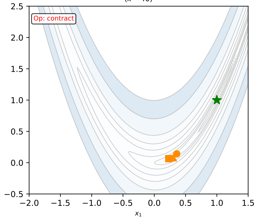
Valley traversal ( k = 40 )
