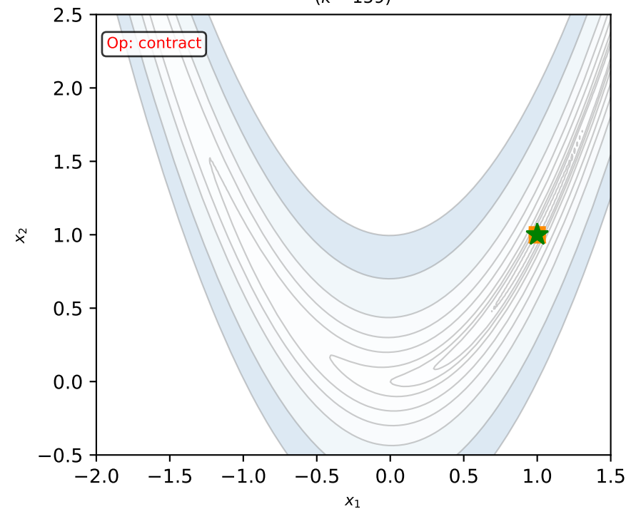
Final simplex ( k = 159 )
