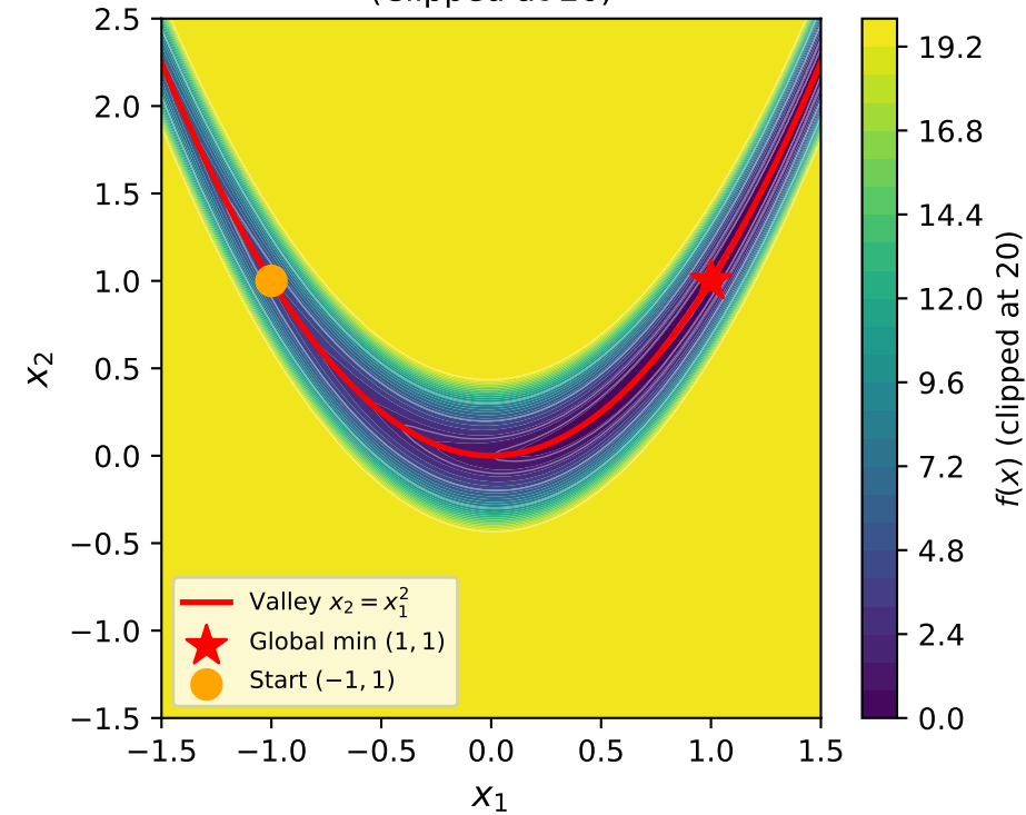
Rosenbrock Function f(x_1, x_2) (Clipped at 20)
