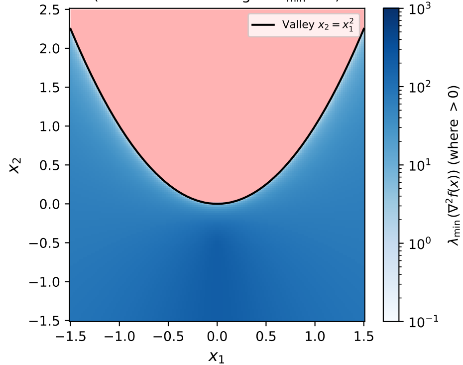
Minimum Eigenvalue \lambda_{\min}(\nabla^2 f) (Red: non-convex region \lambda_{\min} < 0 )
