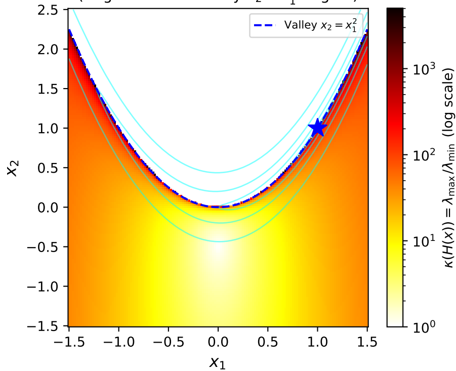
Condition Number \kappa(\nabla^2 f(x)) (Regions above valley x_2 > x_1^2 : high \kappa )
