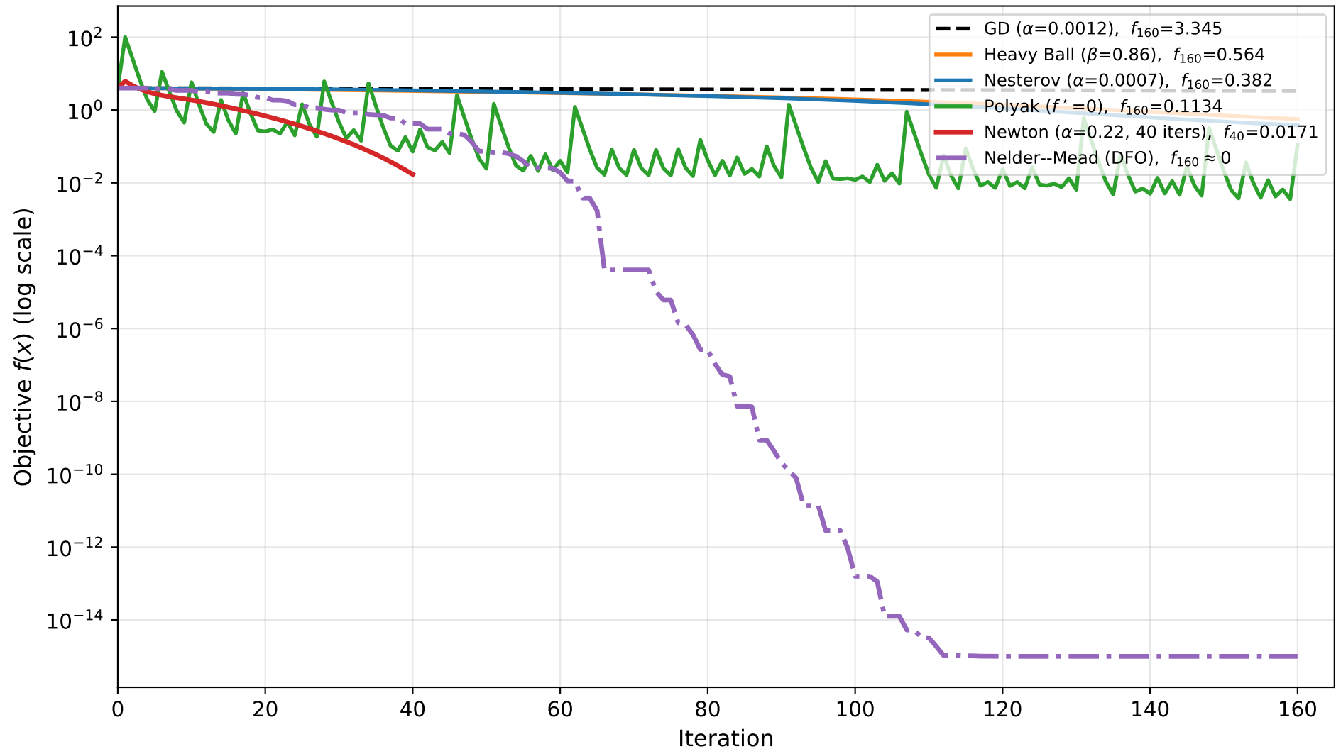
Convergence Comparison Across All Methods — Benchmark C (Rosenbrock)
