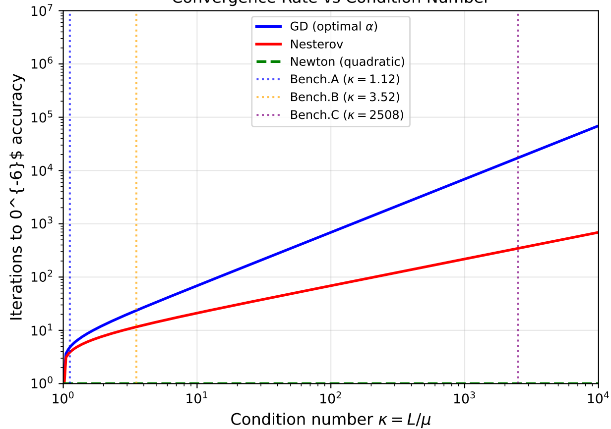
Convergence Rate vs Condition Number
