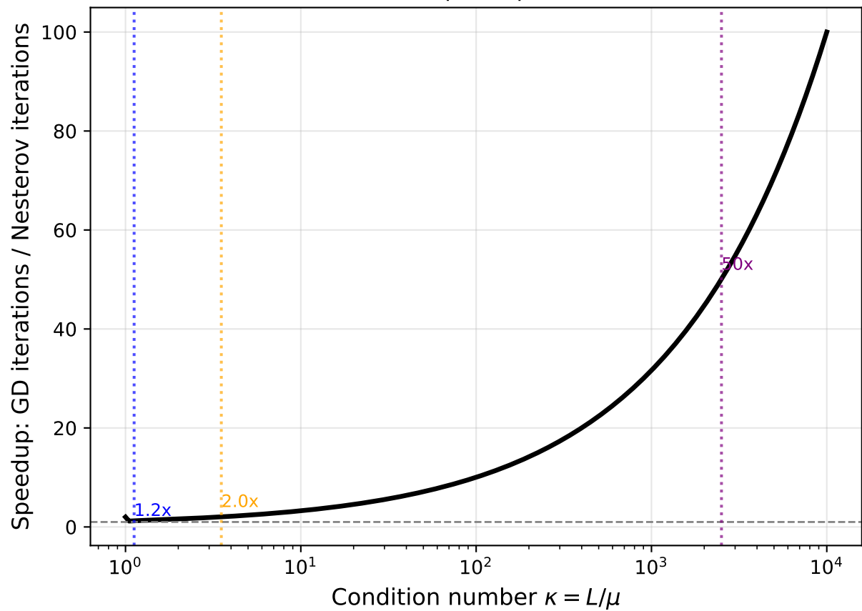
Nesterov Speedup over GD
