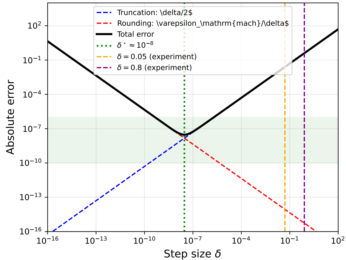
Finite-Difference Error vs \delta
