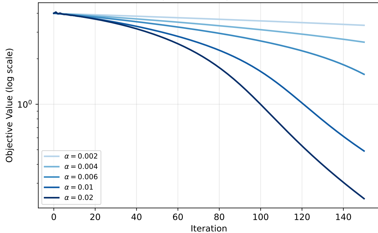
Adam: Sensitivity to Learning Rate \alpha (Rosenbrock)
