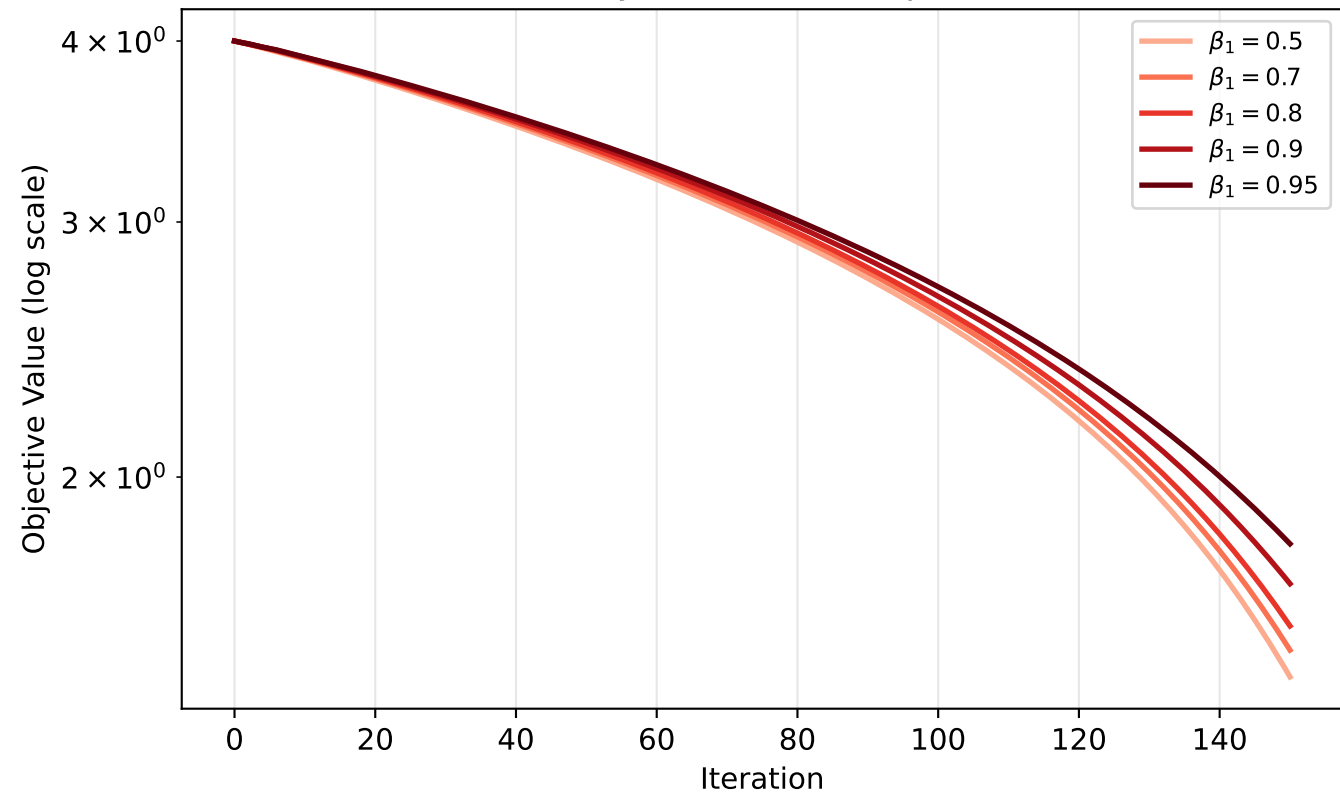
Adam: Sensitivity to Momentum \beta_1 (Rosenbrock)
