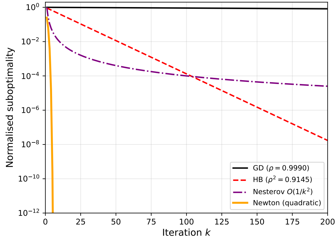
Theoretical convergence rates ( \kappa = 2003 , Rosenbrock)
