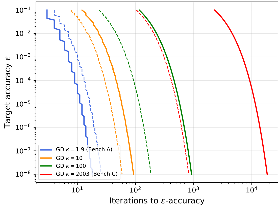
GD (solid) vs Nesterov (dashed) iterations to \varepsilon -accuracy
