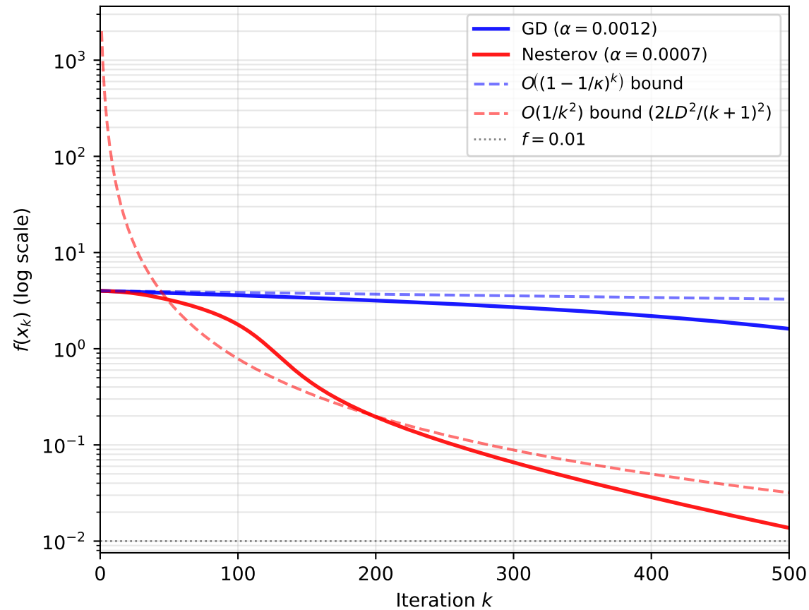
GD vs Nesterov: Rosenbrock ( \kappa \approx 2508 )
