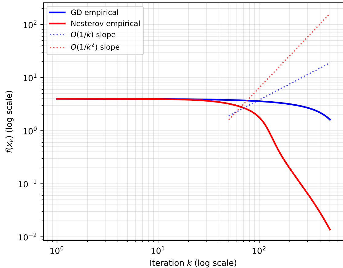
Log-log convergence: slope reveals rate
