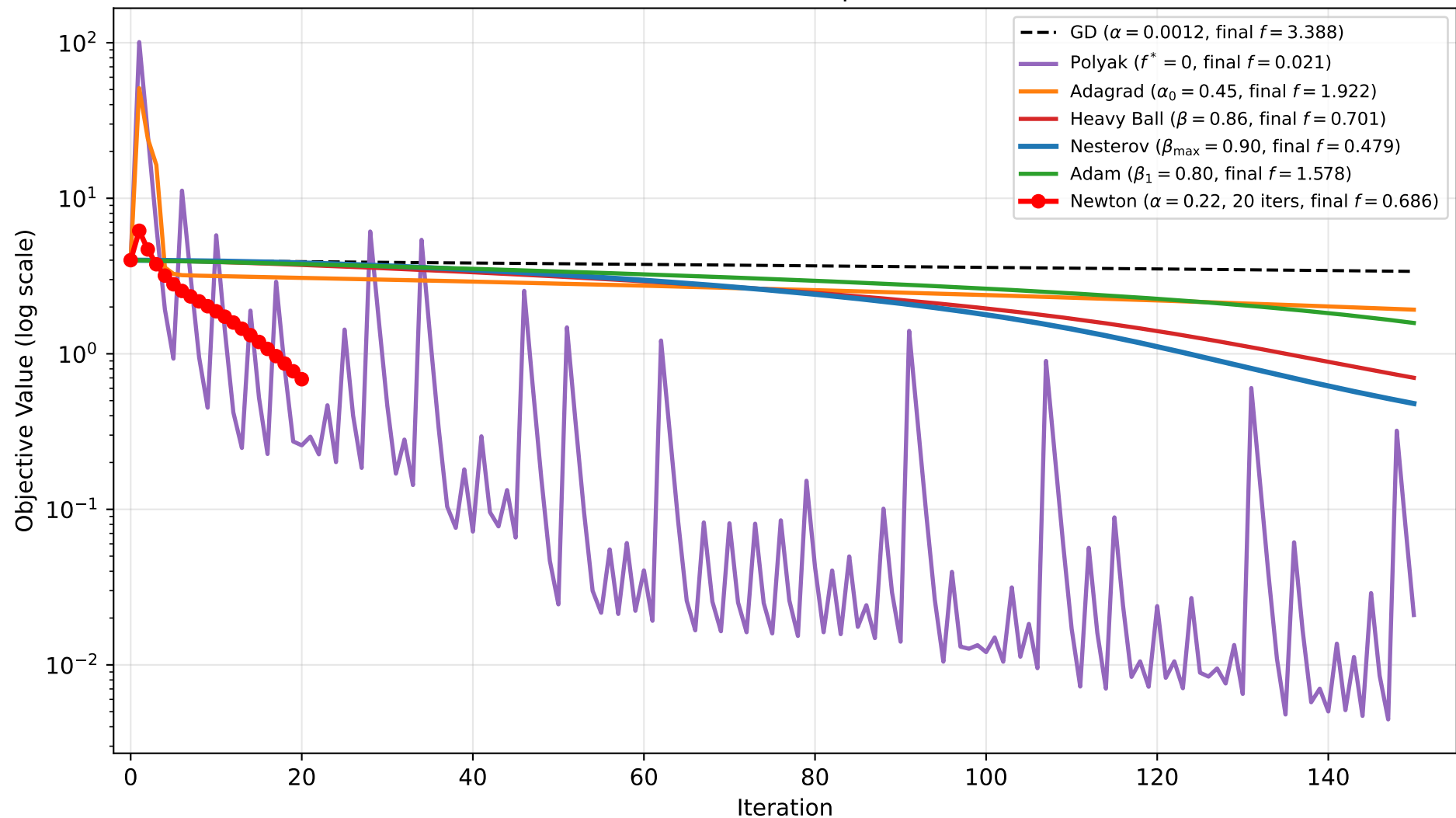
Rosenbrock: All Methods Compared (Benchmark C)
