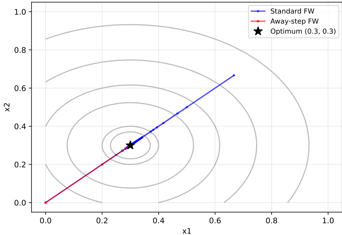
Trajectories on Box [0, 1]^2
