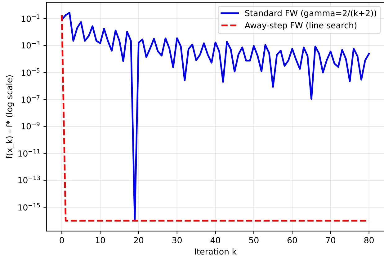
Standard FW vs Away-step FW ( f(x) = ||x - (0.3, 0.3)||^2 , box [0, 1]^2 )
