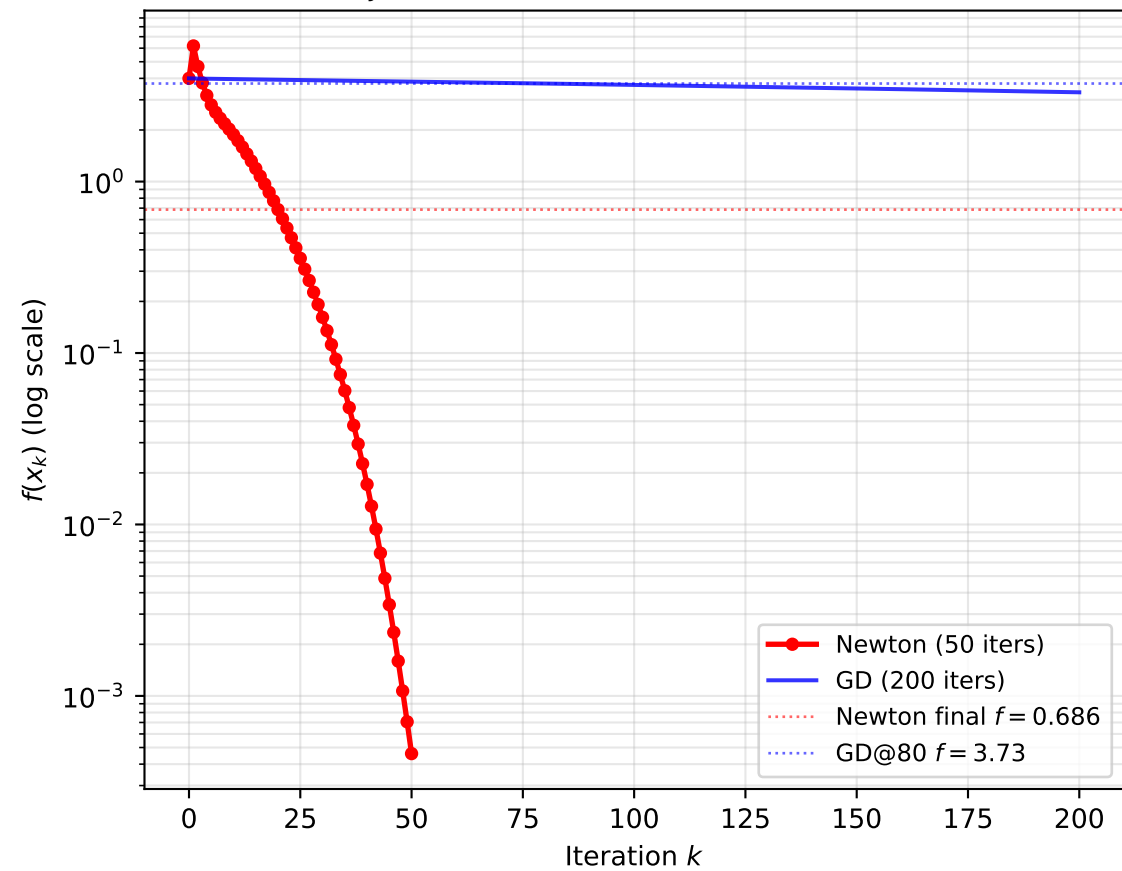
Objective: Newton vs GD (Rosenbrock)
