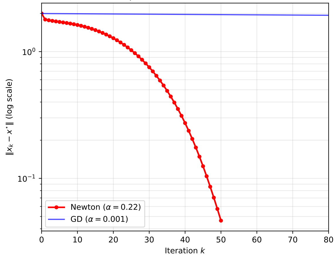
Distance to optimum: Newton vs GD (Rosenbrock)
