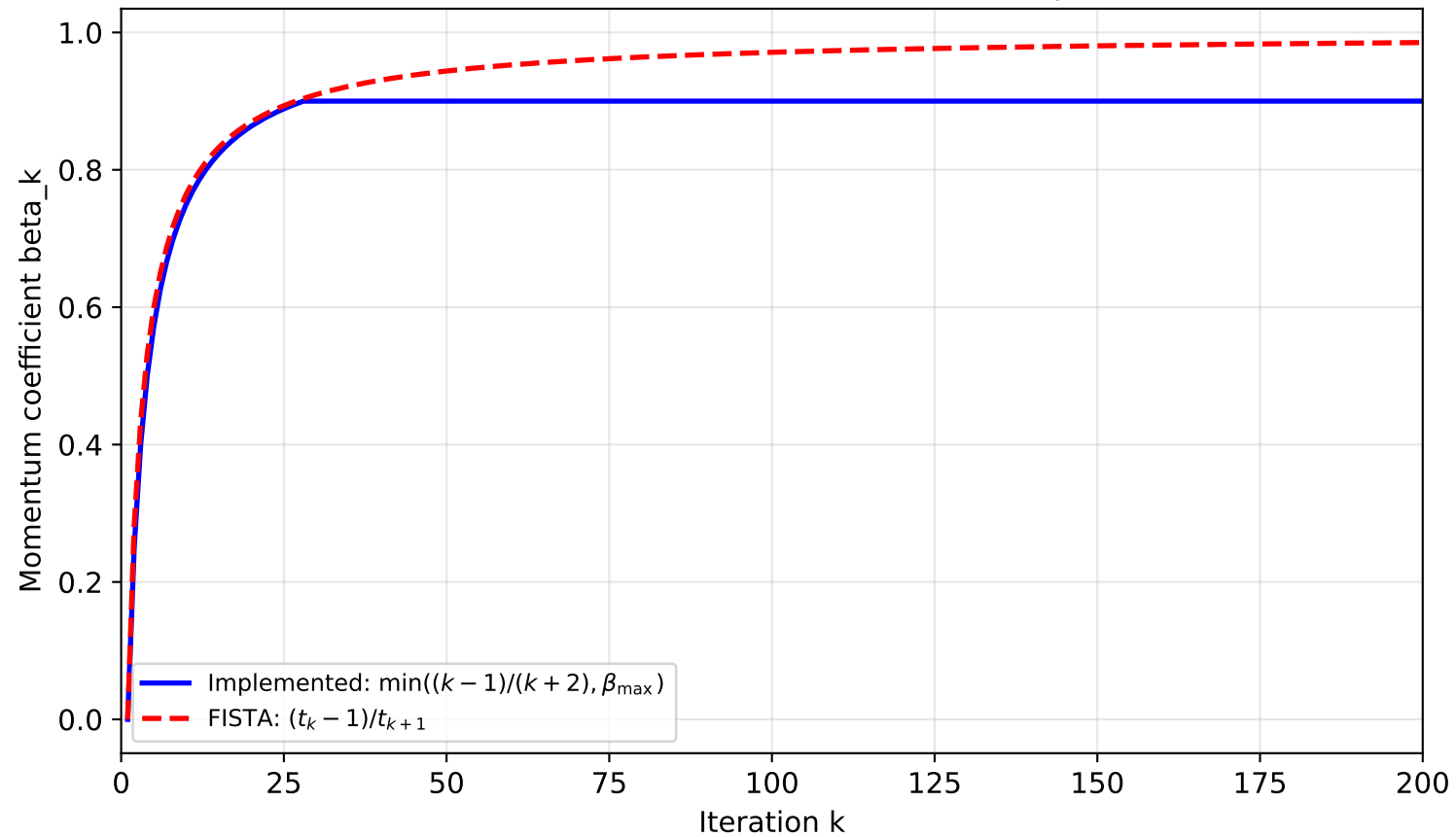
Q2: Nesterov Momentum Schedule Comparison
