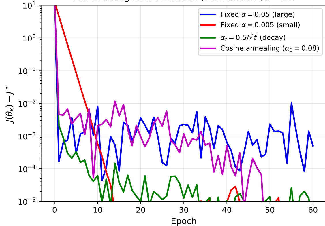
SGD Learning Rate Schedules (Benchmark A, b = 10 )
