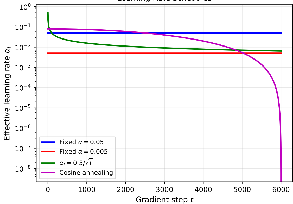
Learning Rate Schedules
