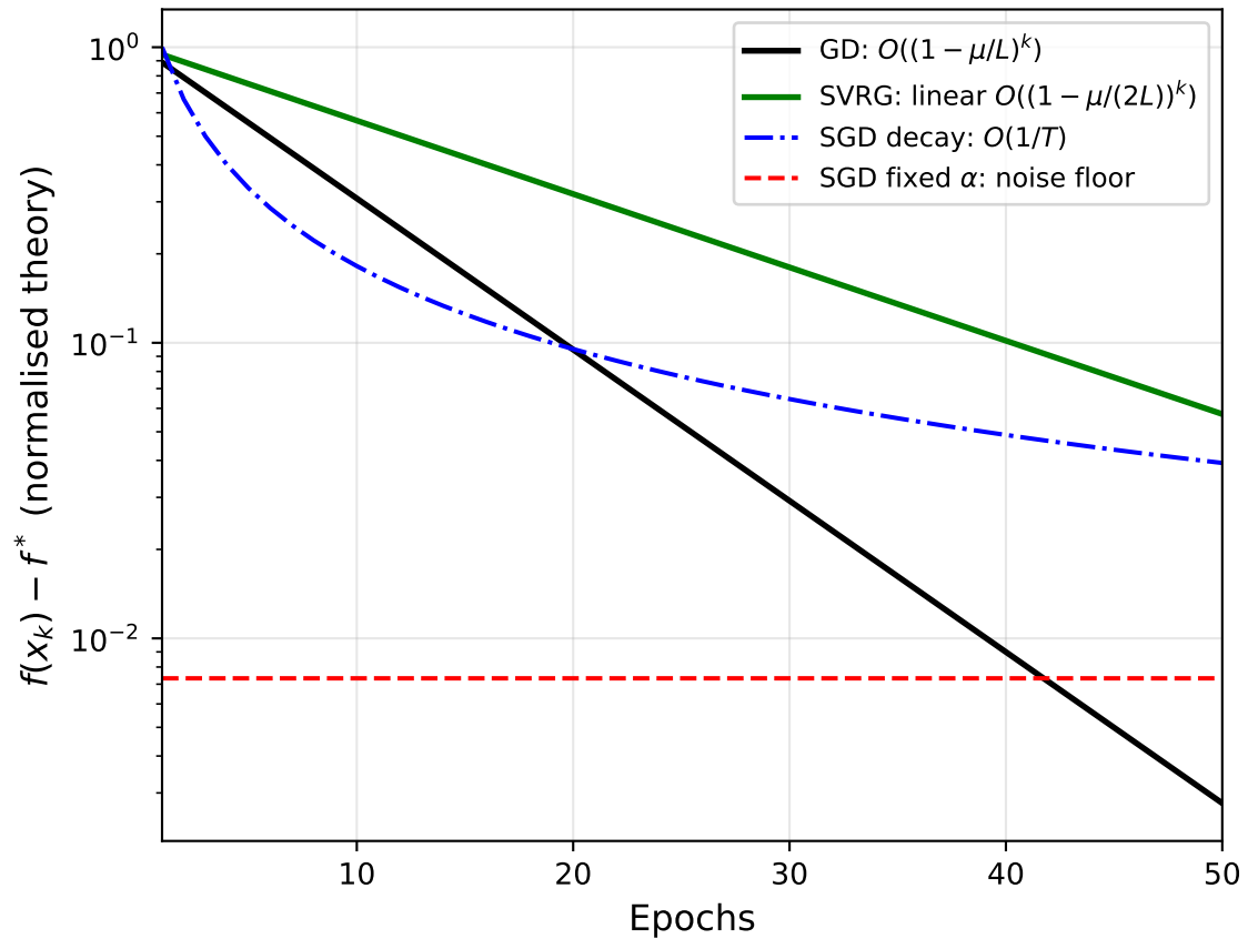
Theoretical Convergence Comparison
