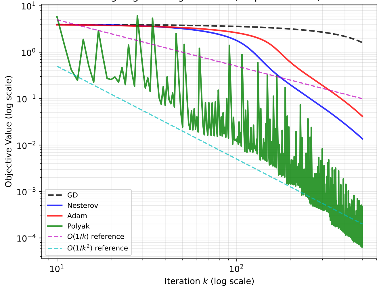
Log-Log Convergence Plot (Empirical Rates)
