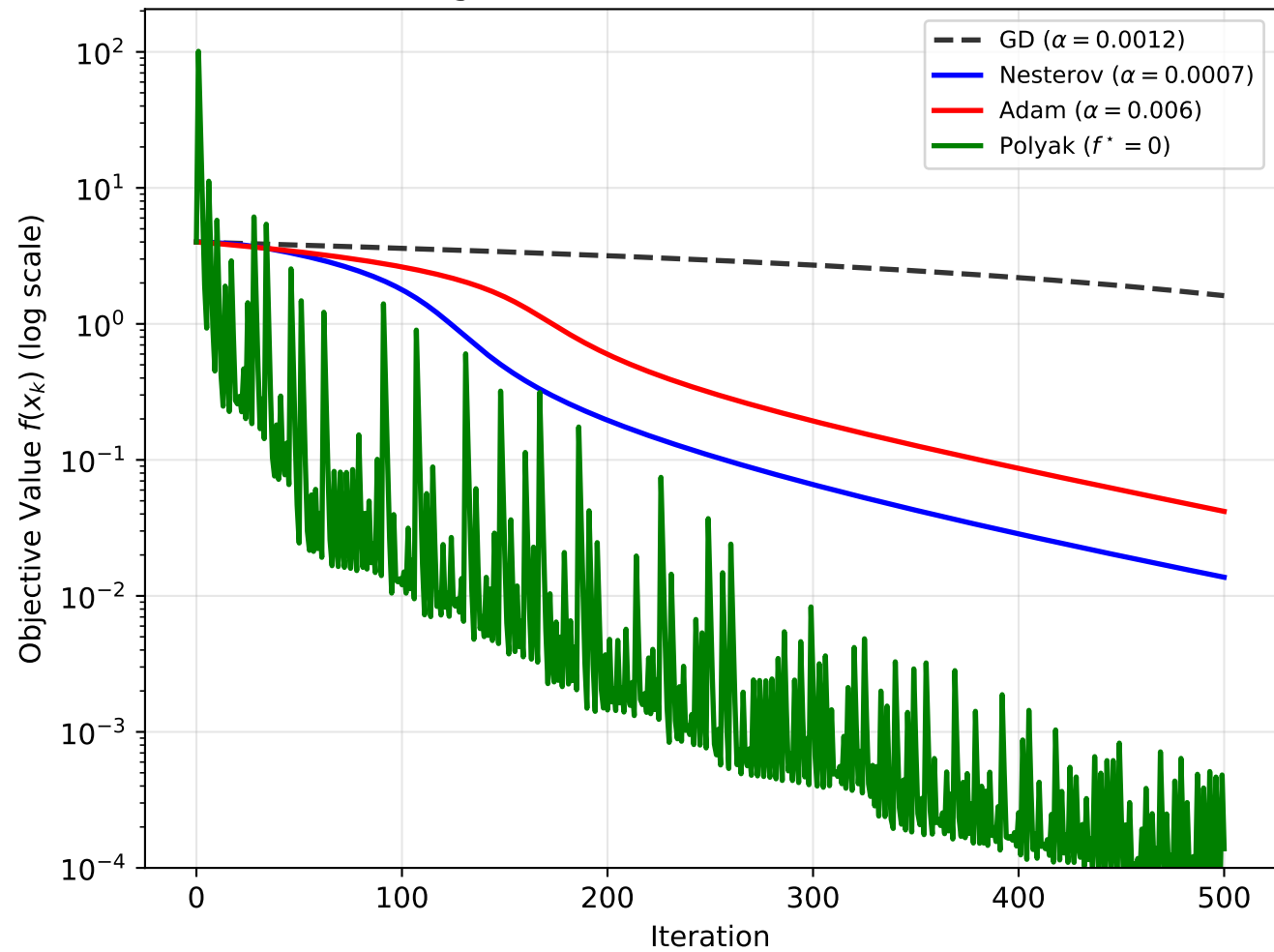
Convergence on Rosenbrock (500 iterations)
