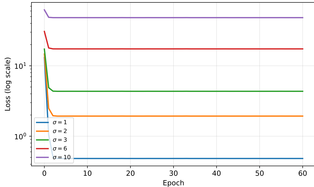
SGD (b=40) convergence for different noise levels \sigma
