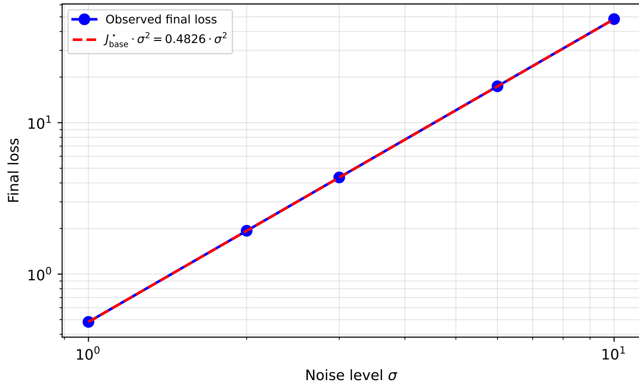
Noise floor scaling: J^* \propto \sigma^2
