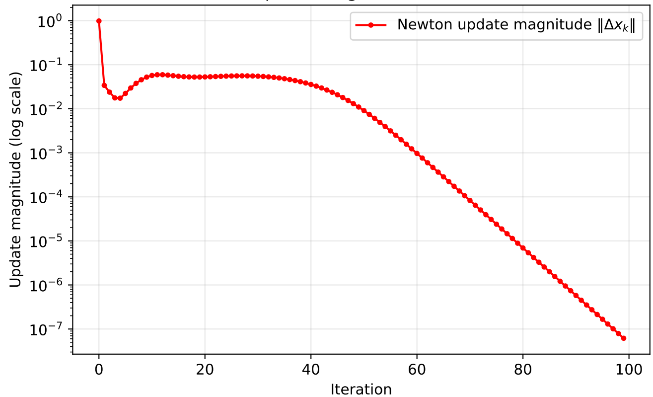
Newton Update Magnitudes (Rosenbrock)
