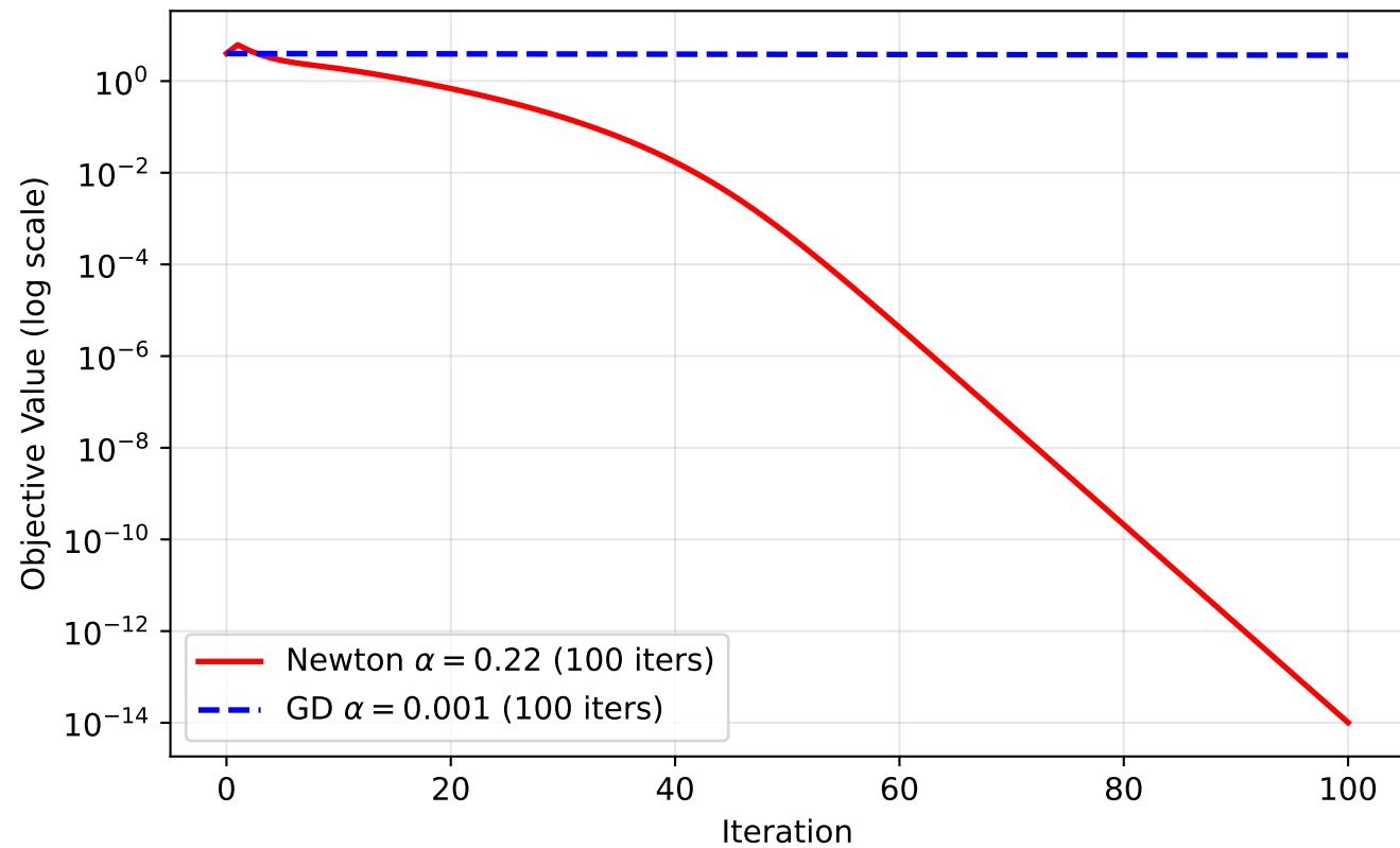
Newton vs GD on Rosenbrock (Extended)
