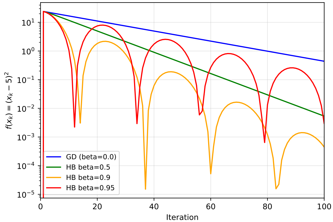
Heavy Ball convergence on quadratic (alpha=0.01)
