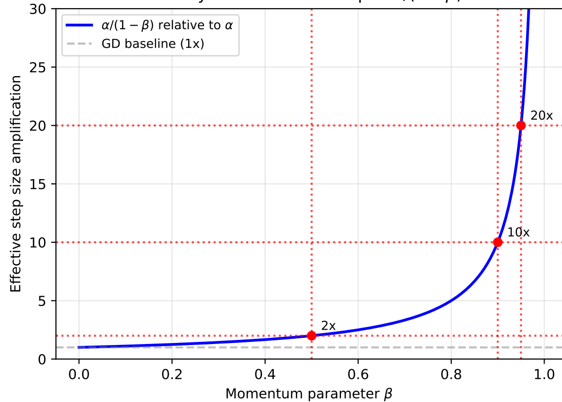
Heavy Ball: Effective Step = \alpha/(1 - \beta)
