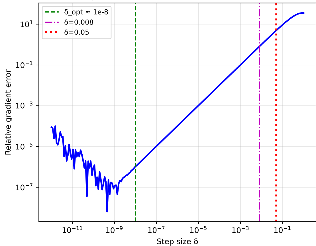
FD gradient error at x_0=(-1,1) on Rosenbrock
