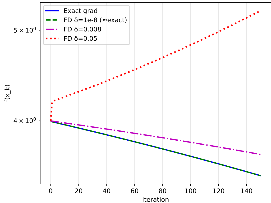
FD GD vs Exact GD on Rosenbrock (Benchmark C)
