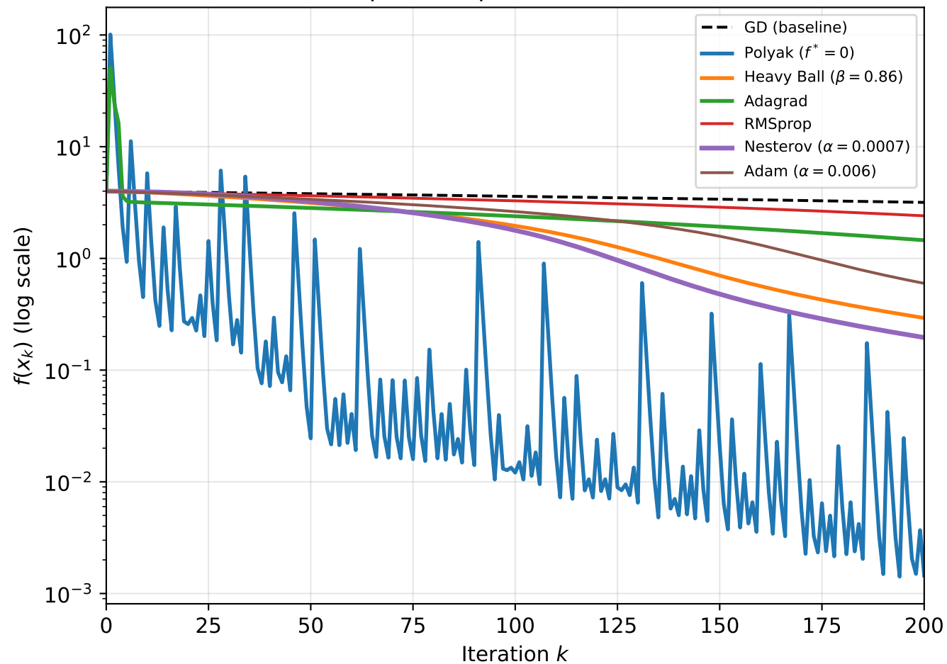
Rosenbrock: All First-Order Methods (Q1: Adaptive step-size; Q2: Momentum)
