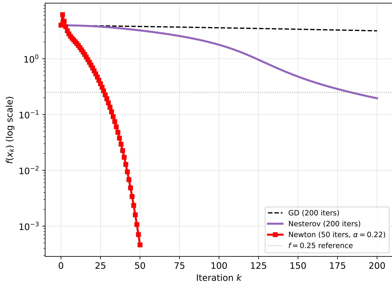
Rosenbrock: First-Order vs Second-Order (Q2 Nesterov vs Q3 Newton)
