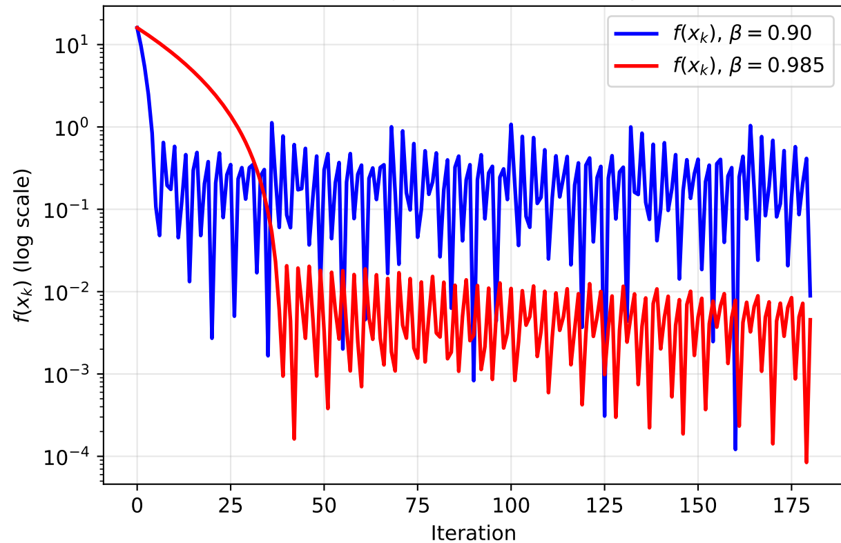
Q6: Primal Objective — Interior Optimum
