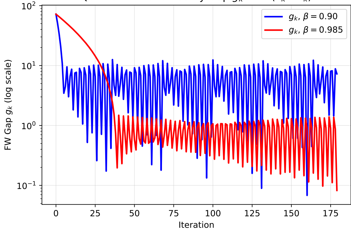
Q6: Frank--Wolfe Duality Gap g_k = \nabla f^T(x_k - z_k)
