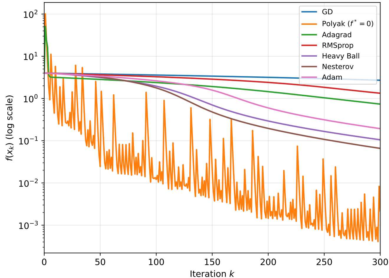
All Q1+Q2 Methods: Convergence on Benchmark C (Full 300 iterations, log scale)
