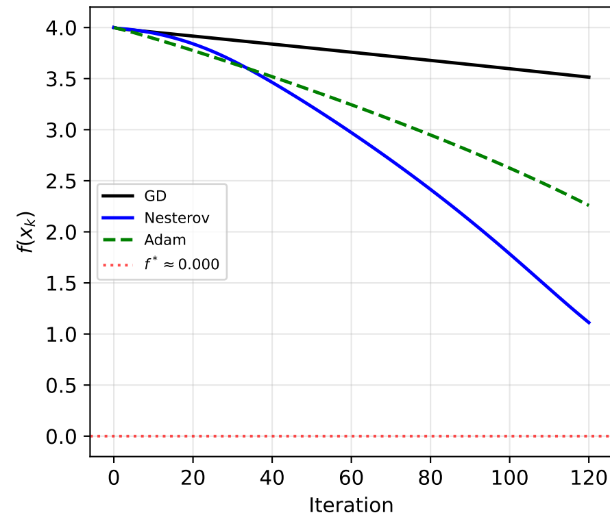
Benchmark C
