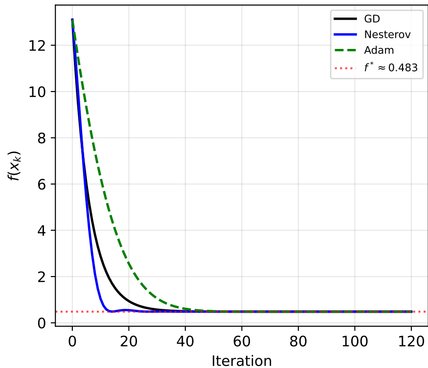
Benchmark A
