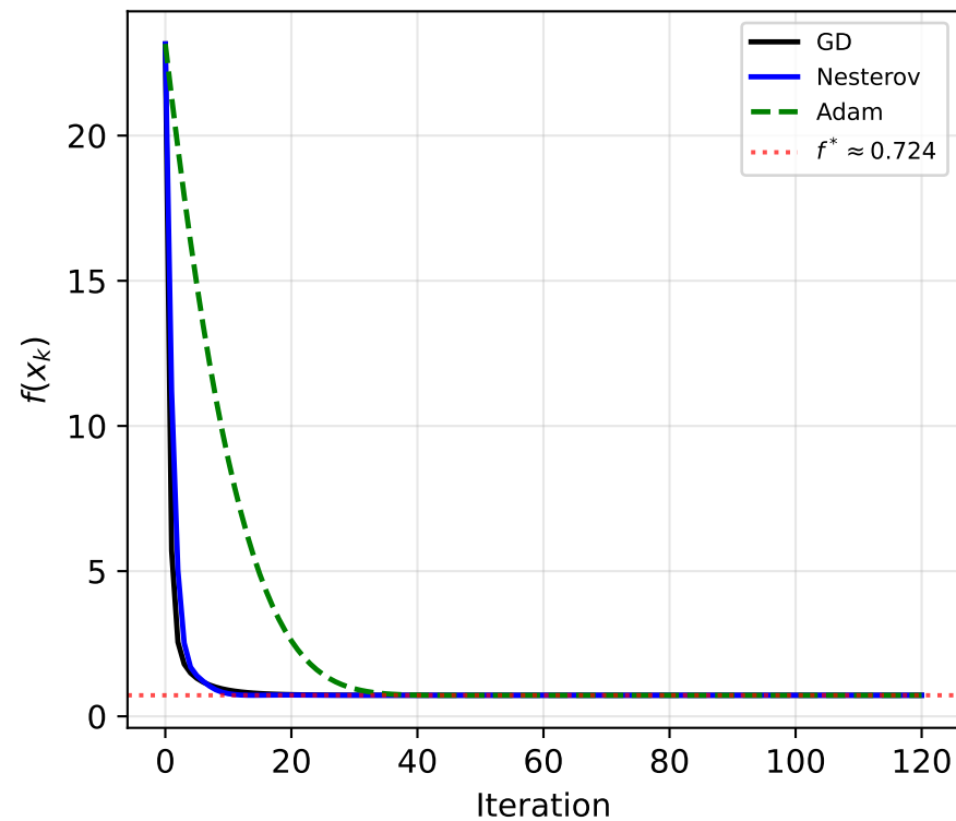
Benchmark B
