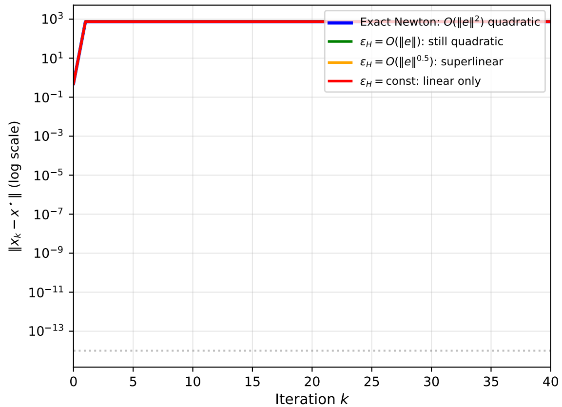
Inexact Newton: Effect of Hessian Approximation Error \varepsilon_H
