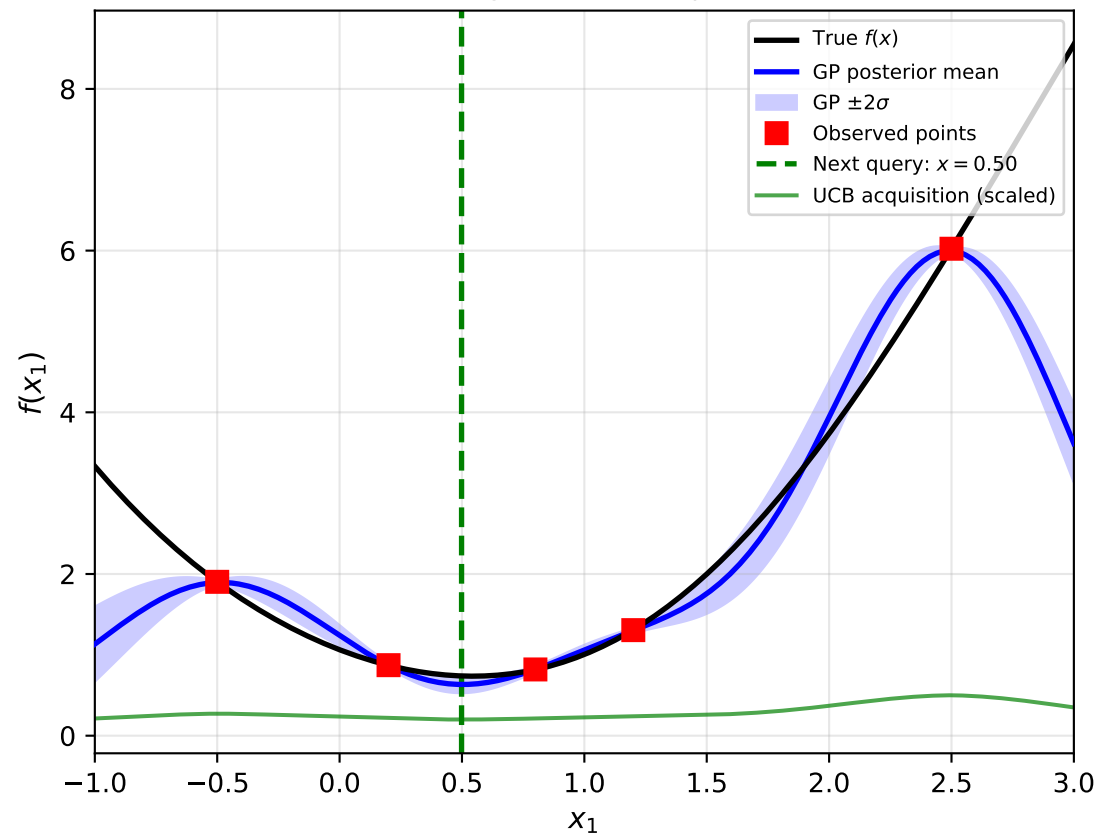
Bayesian Optimization (GP surrogate + UCB acquisition)
