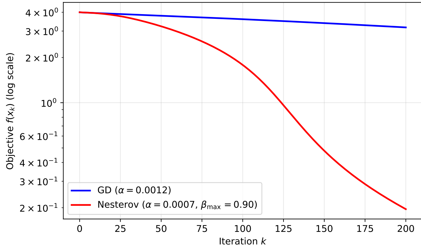
Convergence on Benchmark C (Rosenbrock)
