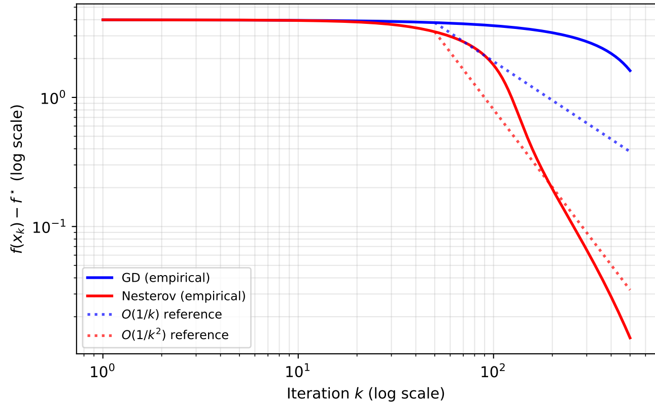
Log-Log Rate: GD O(1/k) vs Nesterov O(1/k^2)
