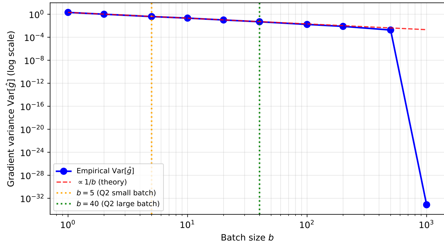
Q2: SGD Gradient Variance vs Batch Size (Benchmark A evaluated at \theta^* , 300 trials/batch)
