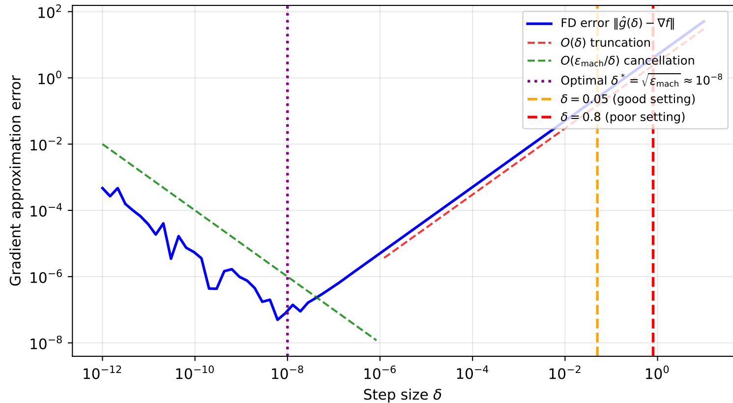
Q4: Finite Difference Gradient Error vs \delta (Benchmark B evaluated at x = (0.5, 2.5) )
