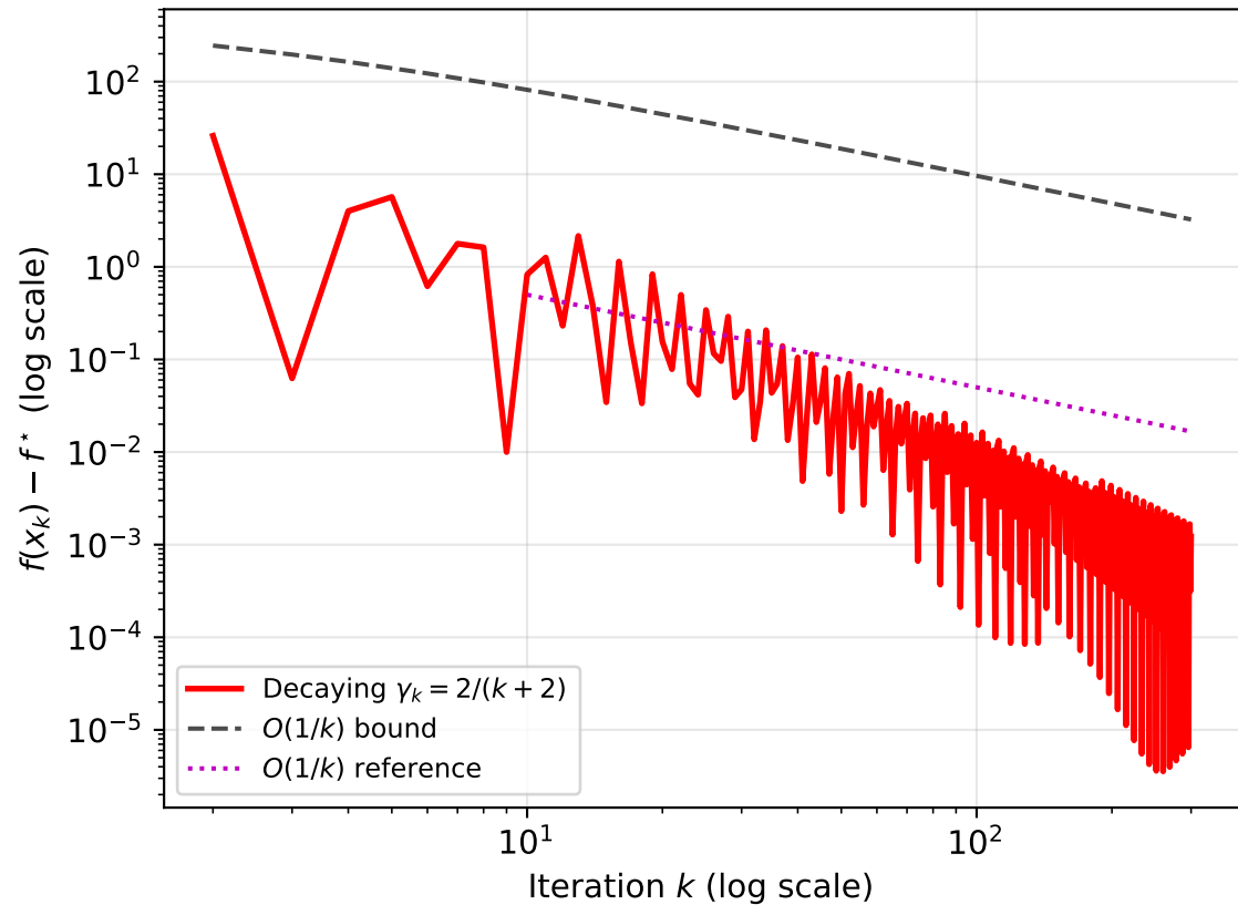
Frank--Wolfe Rate: Log--Log Decaying Schedule
