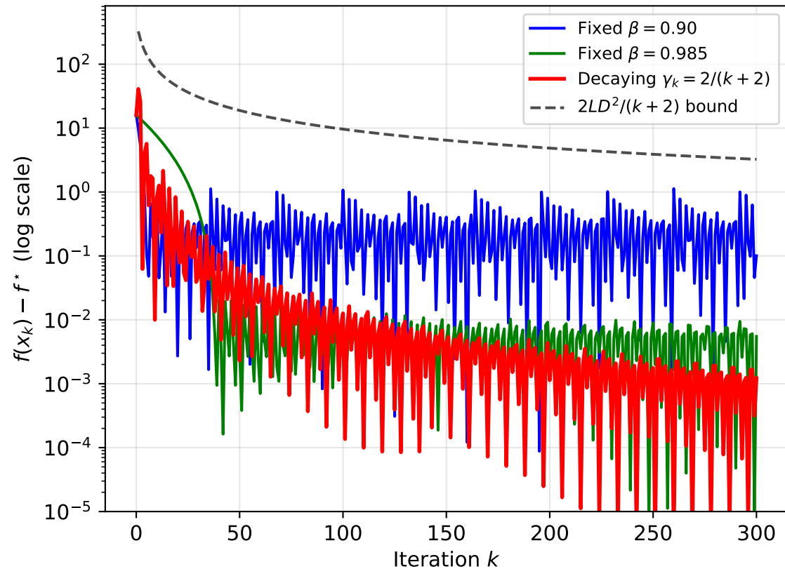
Frank--Wolfe: Interior Optimum Decaying vs Fixed Step
