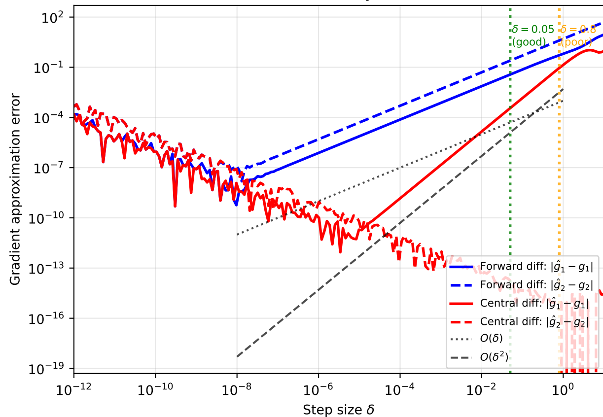
Finite Difference Accuracy on Benchmark B
