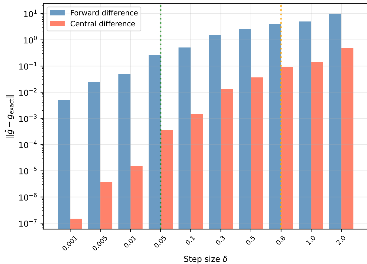
Gradient Approximation Error at Specific \delta Values
