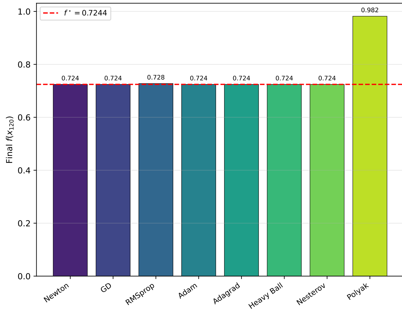
Benchmark B: Final Objective (120 iters)
