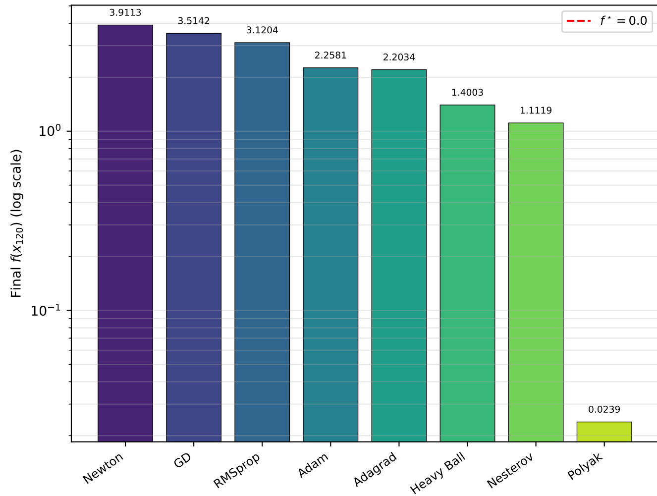
Benchmark C: Final Objective (120 iters, log scale)
