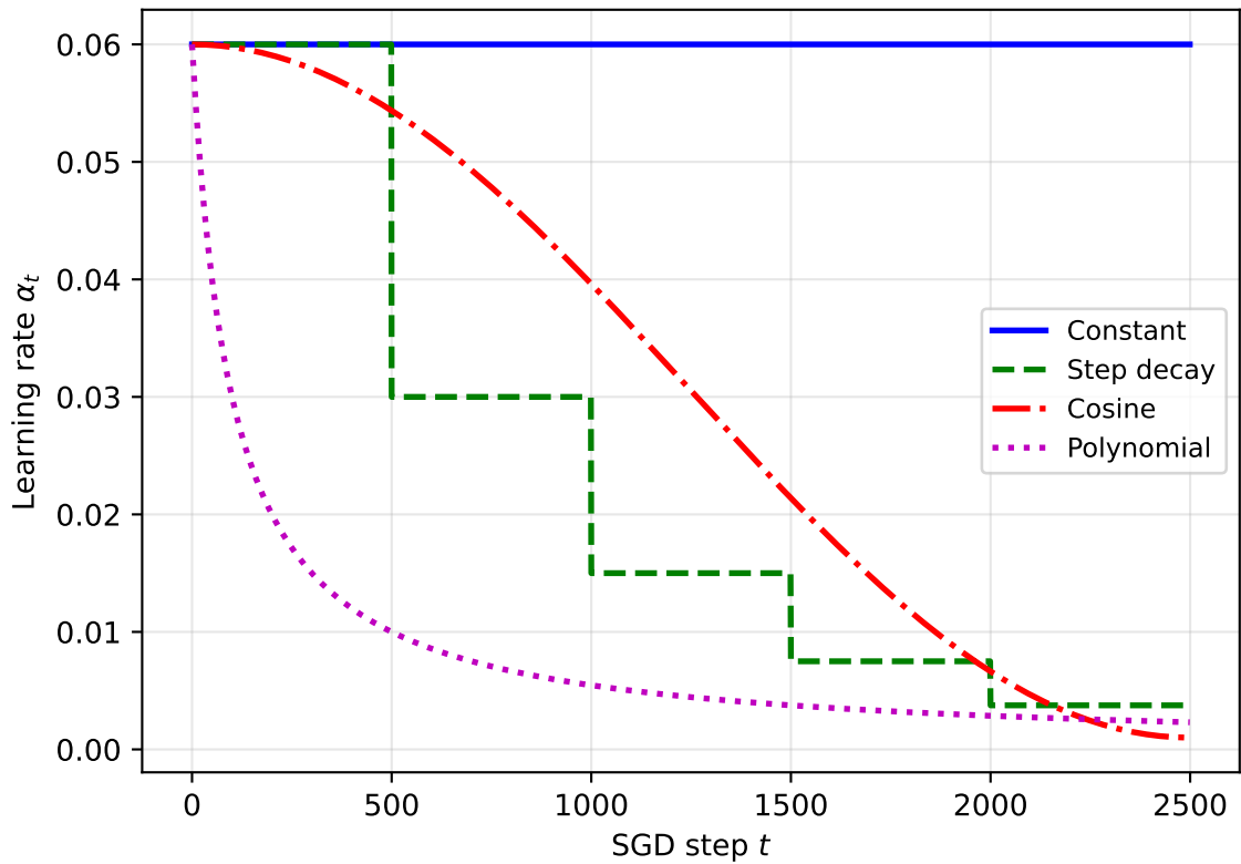
Learning Rate Schedule Values
