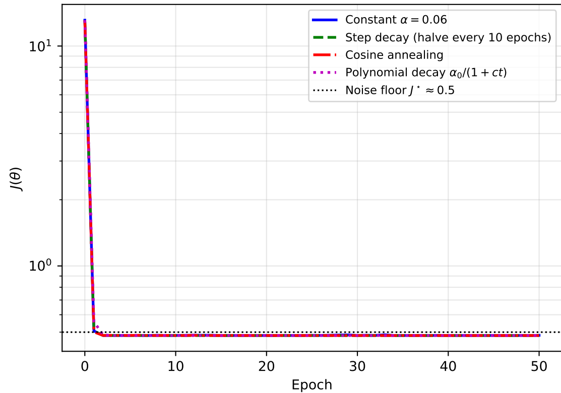
Mini-Batch SGD: Learning Rate Schedule Comparison (Benchmark A, batch=20, 50 epochs)
