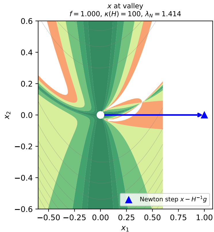
Newton Step Accuracy: Where Quadratic Model Approximates Rosenbrock (green = accurate, red = inaccurate; blue arrow = Newton step)
