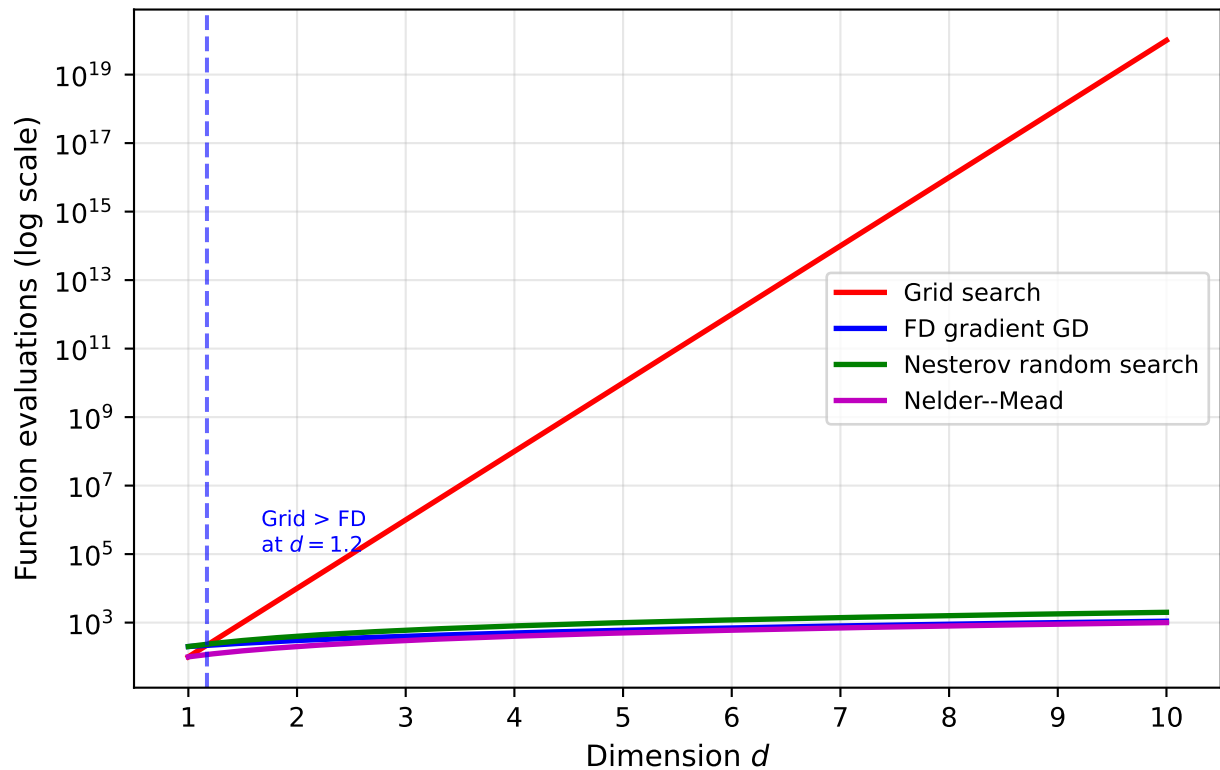
Method Crossover with Dimension (when does each method dominate?)
