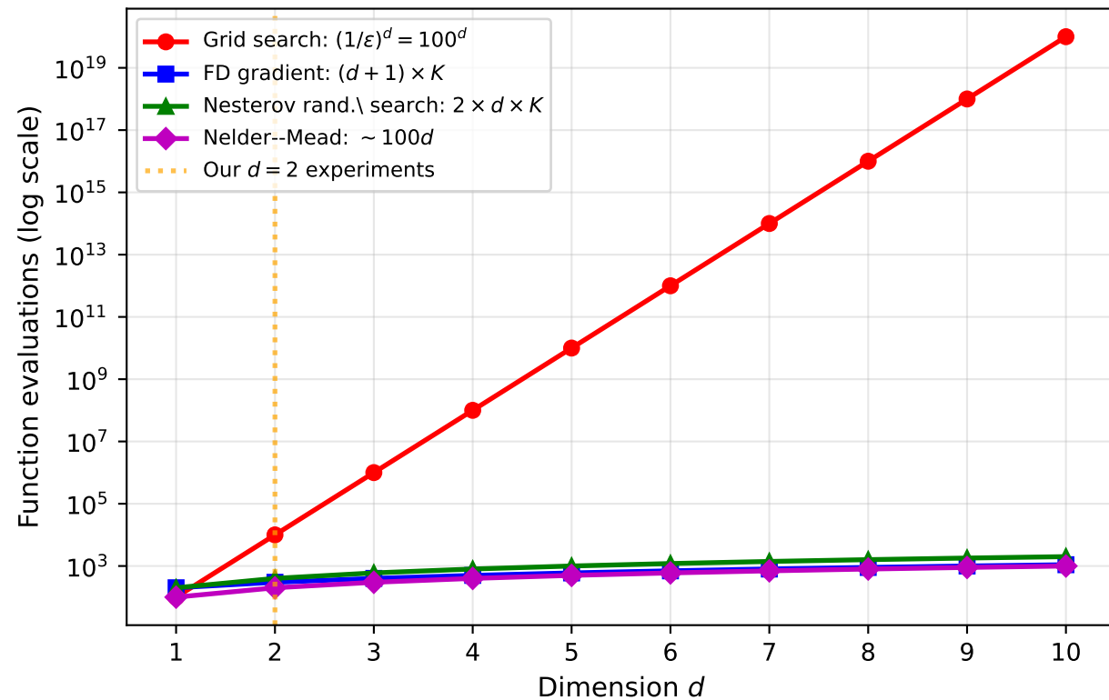
Curse of Dimensionality (function evaluations to \varepsilon = 0.01 accuracy)
