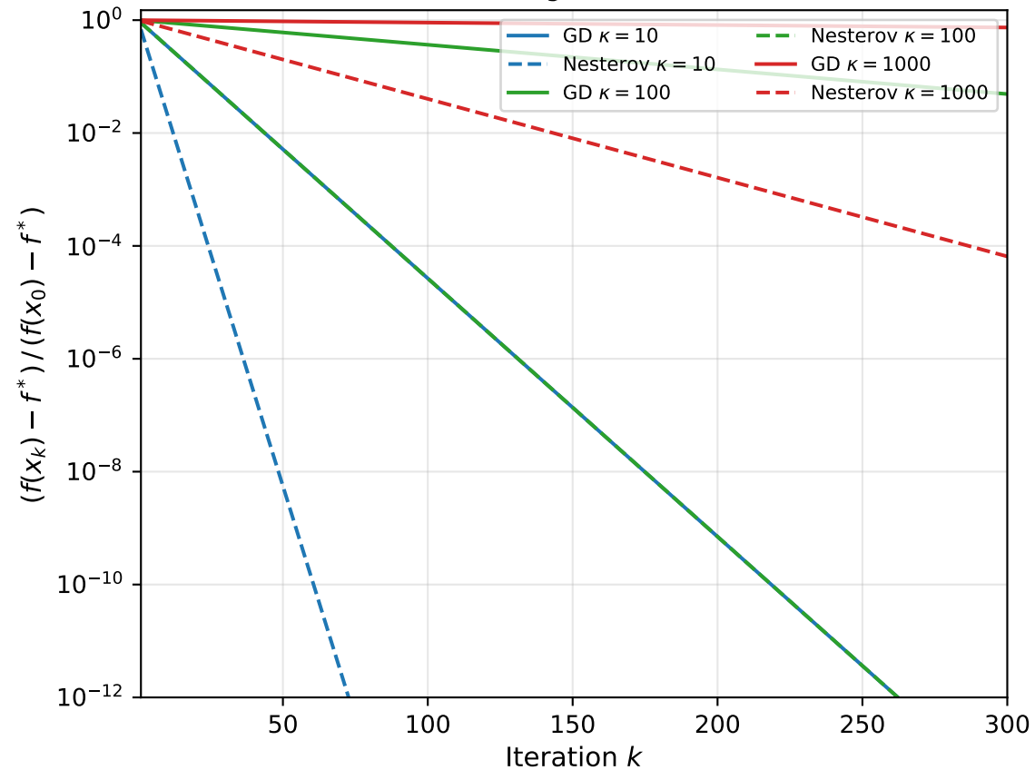
Theoretical convergence: GD vs Nesterov
