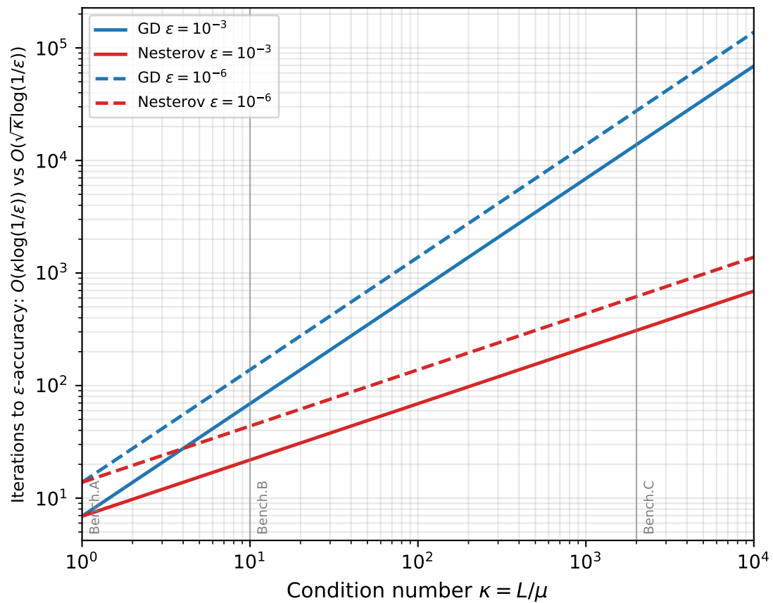
Iterations to converge: GD ( O(\kappa) ) vs Nesterov ( O(\sqrt{\kappa}) )
