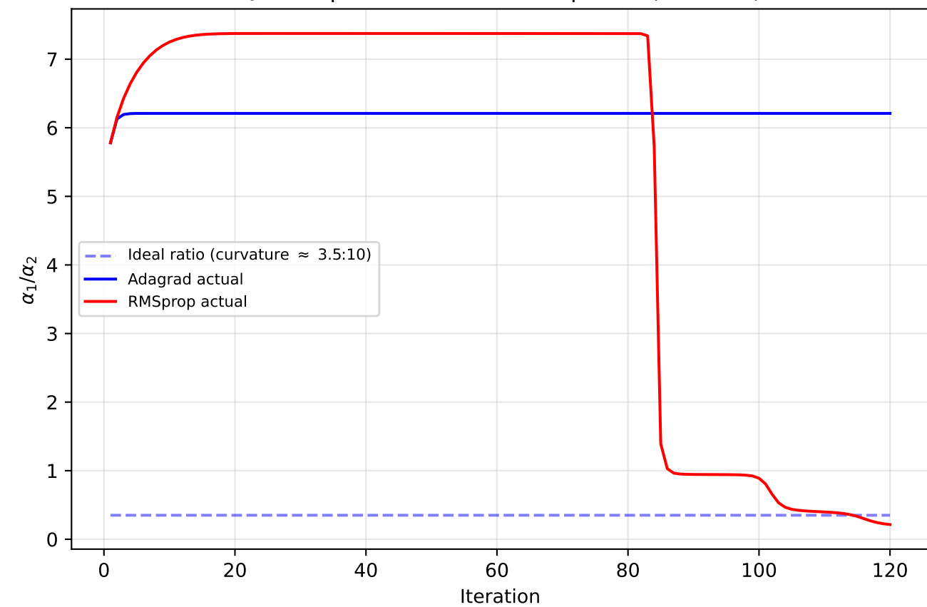
Q1: Adaptive Rate Ratio vs Optimal (Bench B)
