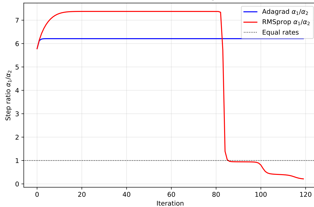
Q1: Ratio of Per-Coordinate Learning Rates ( x_1/x_2 )
