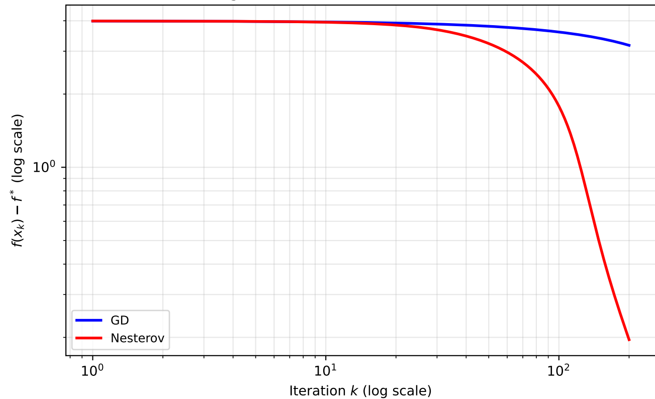
Convergence Rate: Benchmark C (Rosenbrock)
