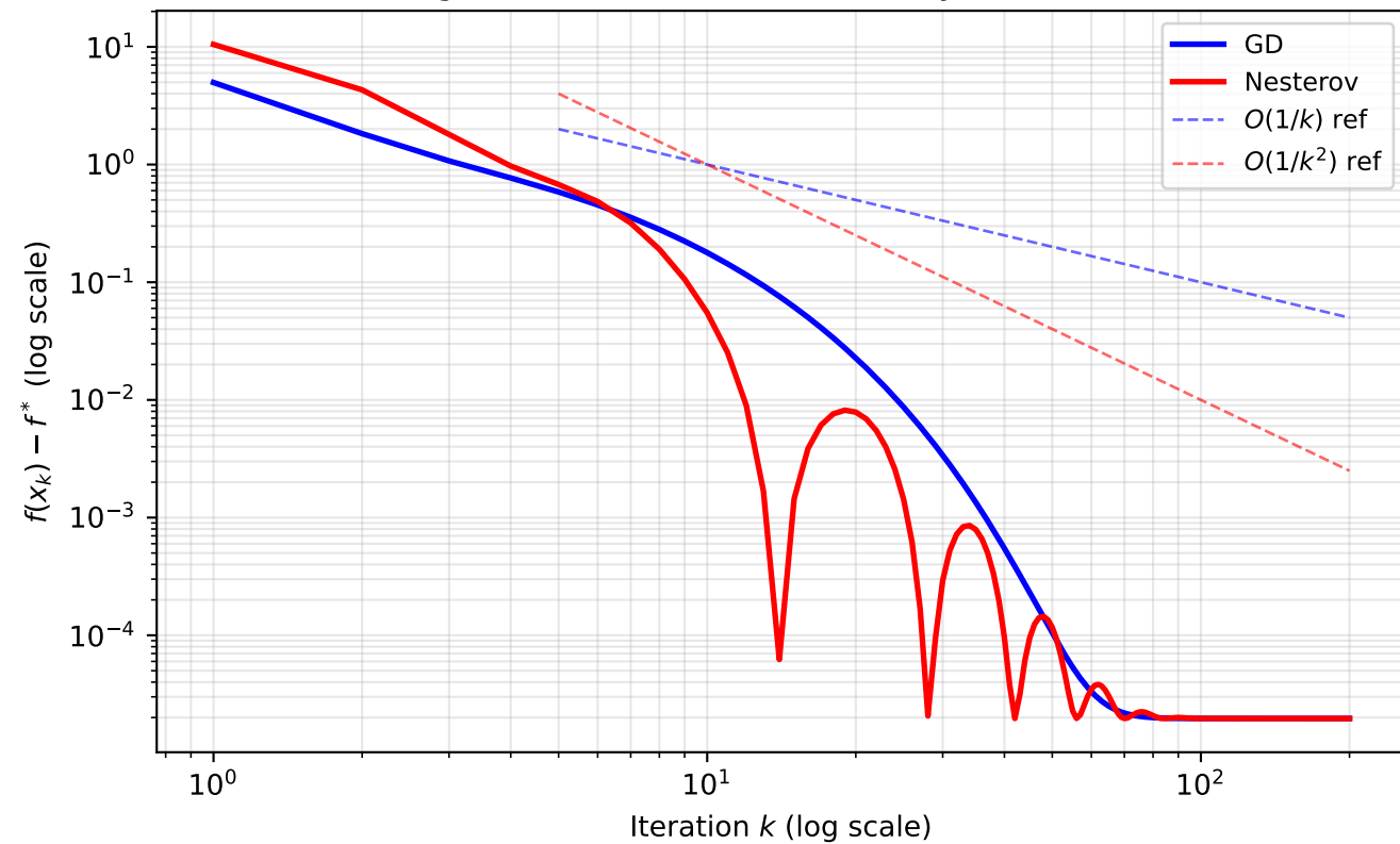
Convergence Rate: Benchmark B (Toy Neural Network)
