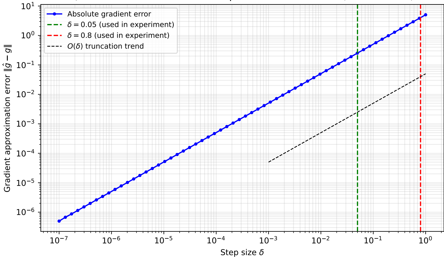
Q4: Finite Difference Error vs Step Size \delta at a Test Point (Benchmark B)
