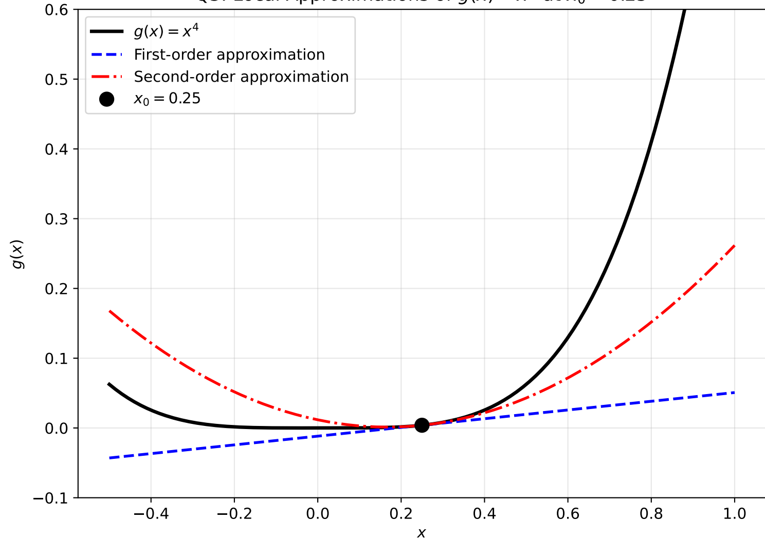
Q3: Local Approximations of g(x) = x^4 at x_0 = 0.25
